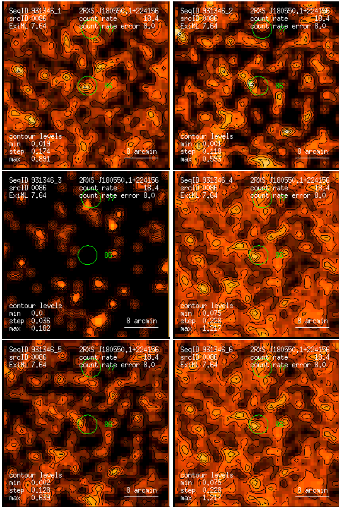
Figure 86: RASS 931346: detection 0086: band rate images, Gaussian filter: (1) PSPC channels 11 – 41, (2) 52 – 90, (3) 91 – 201, (4) 11 – 235, (5) 52 – 201, (6) 11 – 201. Broad band rates in counts/ks. Band rate contour levels in counts/ks/arcmin 2 .
