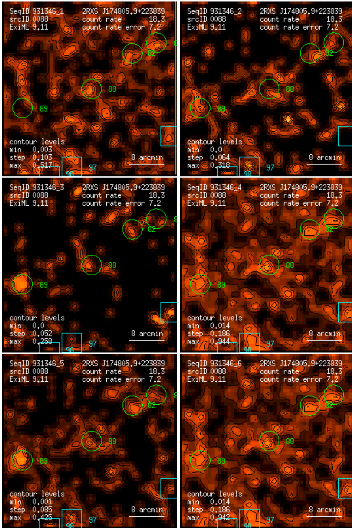
Figure 88: RASS 931346: detection 0088: band rate images, Gaussian filter: (1) PSPC channels 11 – 41, (2) 52 – 90, (3) 91 – 201, (4) 11 – 235, (5) 52 – 201, (6) 11 – 201. Broad band rates in counts/ks. Band rate contour levels in counts/ks/arcmin 2 .
