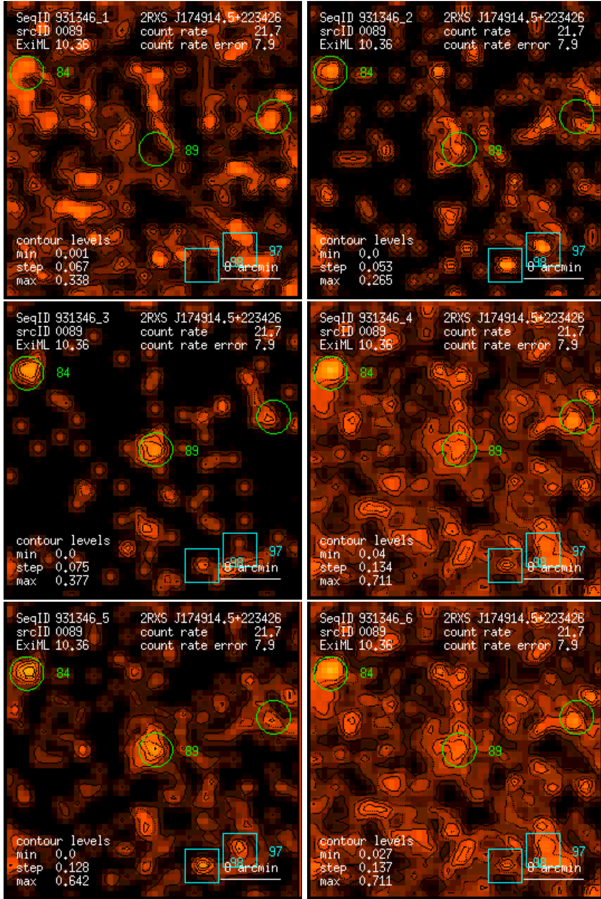
Figure 89: RASS 931346: detection 0089: band rate images, Gaussian filter: (1) PSPC channels 11 – 41, (2) 52 – 90, (3) 91 – 201, (4) 11 – 235, (5) 52 – 201, (6) 11 – 201. Broad band rates in counts/ks. Band rate contour levels in counts/ks/arcmin 2 .
