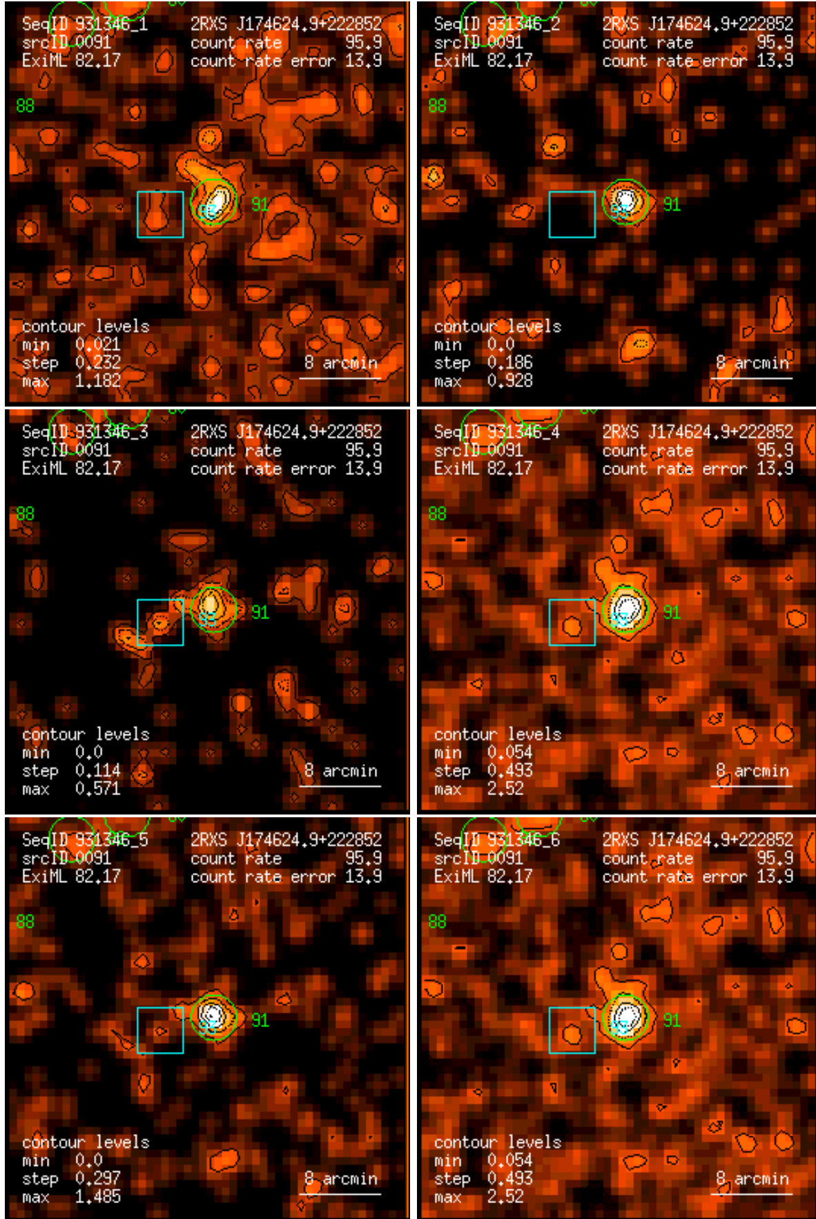
Figure 91: RASS 931346: detection 0091: band rate images, Gaussian filter: (1) PSPC channels 11 – 41, (2) 52 – 90, (3) 91 – 201, (4) 11 – 235, (5) 52 – 201, (6) 11 – 201. Broad band rates in counts/ks. Band rate contour levels in counts/ks/arcmin 2 .
