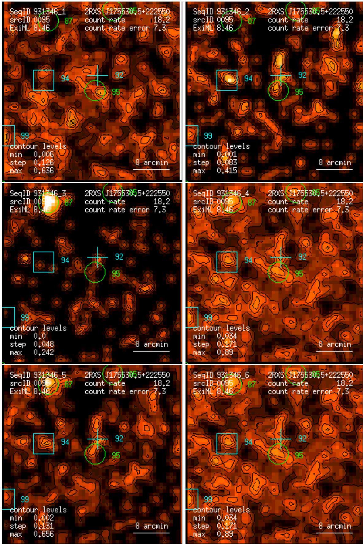
Figure 95: RASS 931346: detection 0095: band rate images, Gaussian filter: (1) PSPC channels 11 – 41, (2) 52 – 90, (3) 91 – 201, (4) 11 – 235, (5) 52 – 201, (6) 11 – 201. Broad band rates in counts/ks. Band rate contour levels in counts/ks/arcmin 2 .
