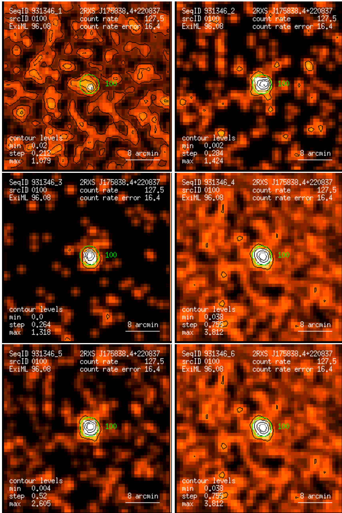
Figure 100: RASS 931346: detection 0100: band rate images, Gaussian filter: (1) PSPC channels 11 – 41, (2) 52 – 90, (3) 91 – 201, (4) 11 – 235, (5) 52 – 201, (6) 11 – 201. Broad band rates in counts/ks. Band rate contour levels in counts/ks/arcmin 2 .
