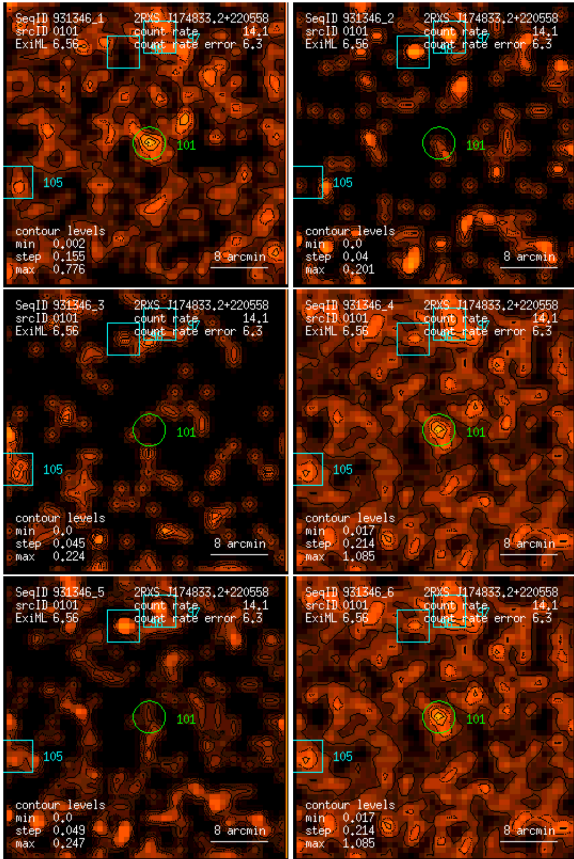
Figure 101: RASS 931346: detection 0101: band rate images, Gaussian filter: (1) PSPC channels 11 – 41, (2) 52 – 90, (3) 91 – 201, (4) 11 – 235, (5) 52 – 201, (6) 11 – 201. Broad band rates in counts/ks. Band rate contour levels in counts/ks/arcmin 2 .
