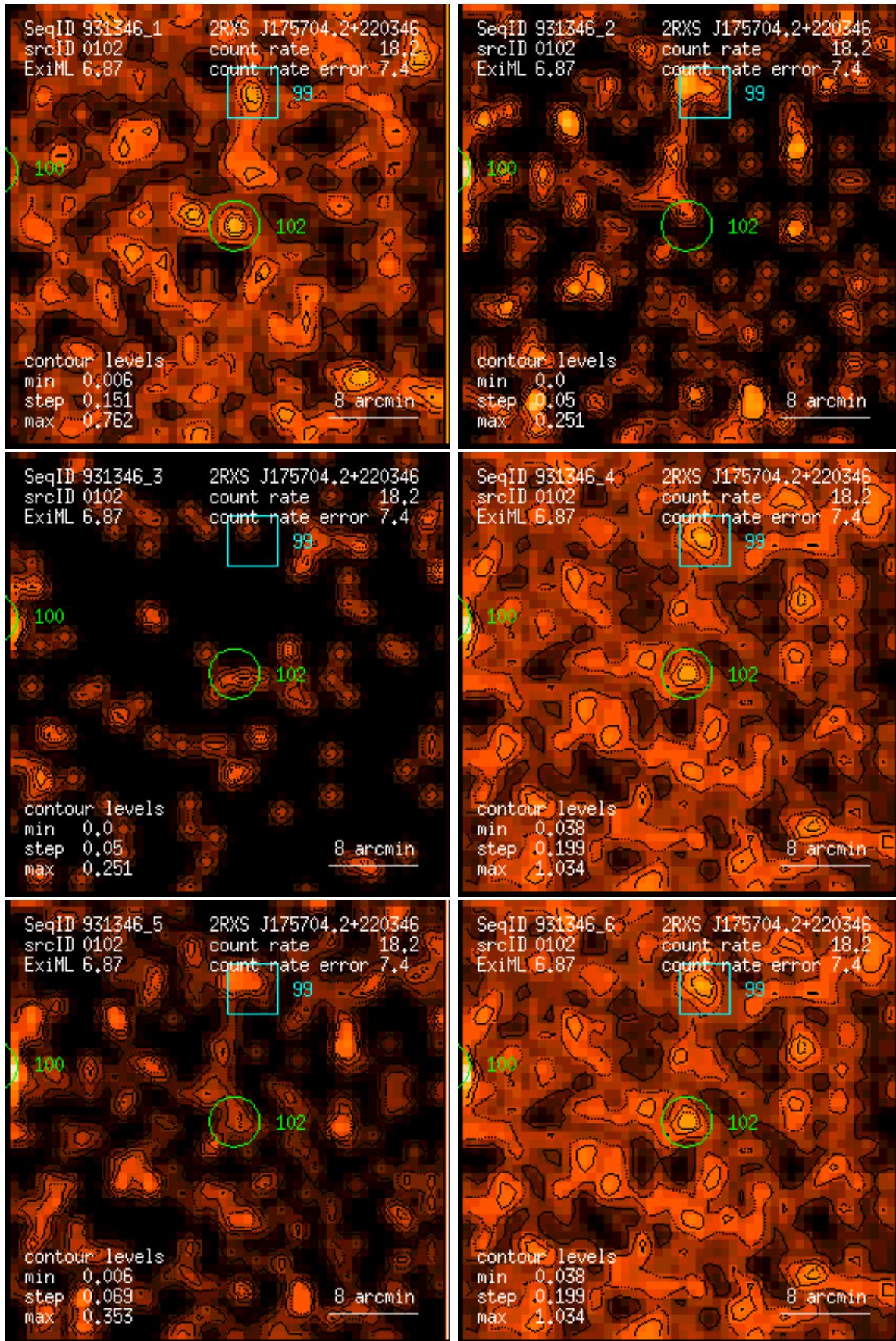
Figure 102: RASS 931346: detection 0102: band rate images, Gaussian filter: (1) PSPC channels 11 – 41, (2) 52 – 90, (3) 91 – 201, (4) 11 – 235, (5) 52 – 201, (6) 11 – 201. Broad band rates in counts/ks. Band rate contour levels in counts/ks/arcmin 2 .
