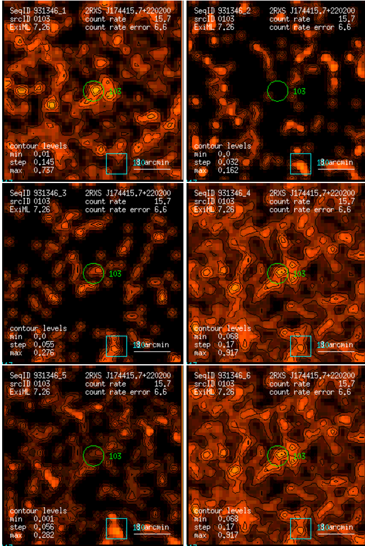
Figure 103: RASS 931346: detection 0103: band rate images, Gaussian filter: (1) PSPC channels 11 – 41, (2) 52 – 90, (3) 91 – 201, (4) 11 – 235, (5) 52 – 201, (6) 11 – 201. Broad band rates in counts/ks. Band rate contour levels in counts/ks/arcmin 2 .
