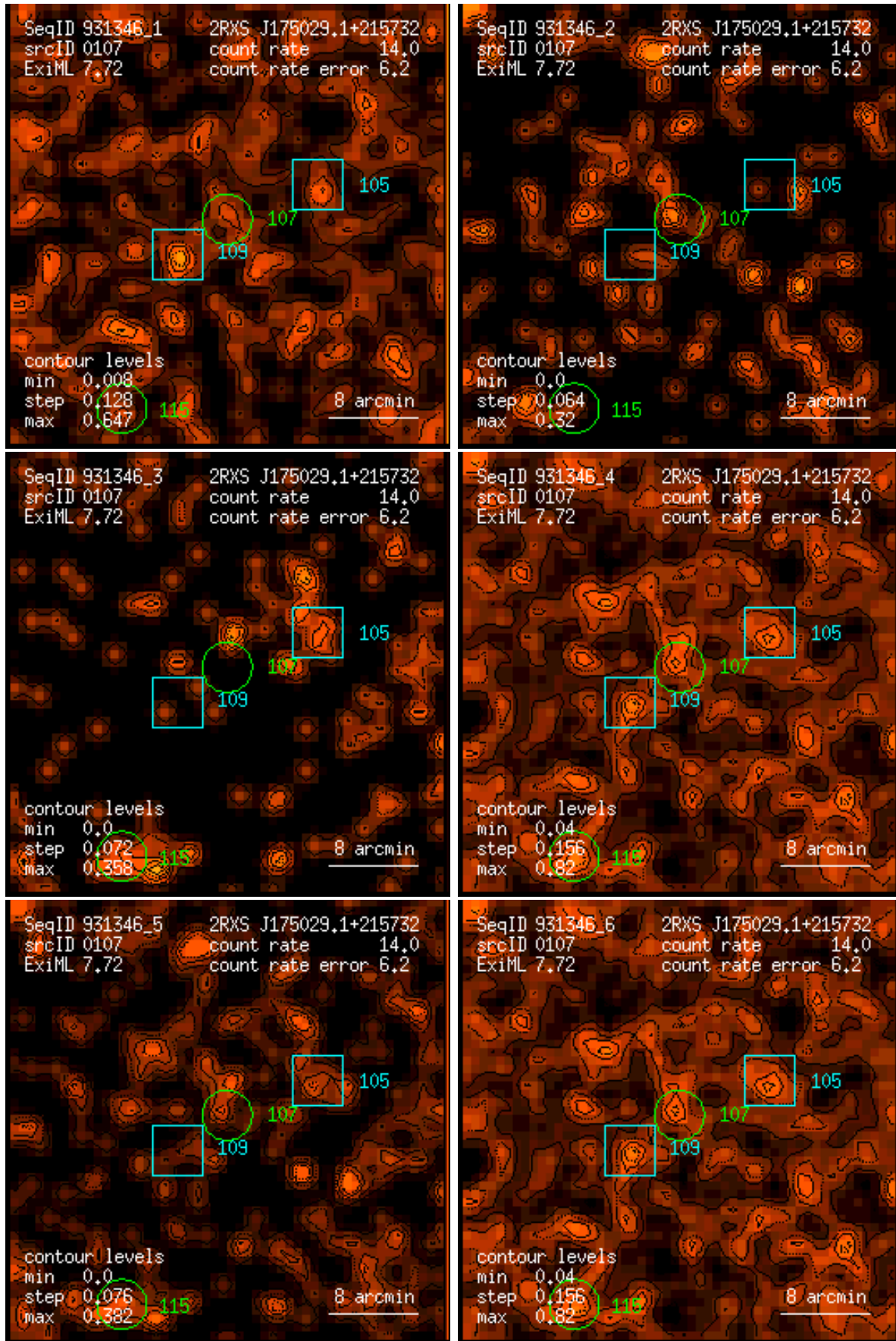
Figure 107: RASS 931346: detection 0107: band rate images, Gaussian filter: (1) PSPC channels 11 – 41, (2) 52 – 90, (3) 91 – 201, (4) 11 – 235, (5) 52 – 201, (6) 11 – 201. Broad band rates in counts/ks. Band rate contour levels in counts/ks/arcmin 2 .
