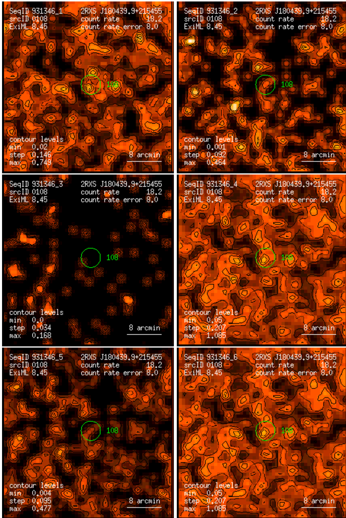
Figure 108: RASS 931346: detection 0108: band rate images, Gaussian filter: (1) PSPC channels 11 – 41, (2) 52 – 90, (3) 91 – 201, (4) 11 – 235, (5) 52 – 201, (6) 11 – 201. Broad band rates in counts/ks. Band rate contour levels in counts/ks/arcmin 2 .
