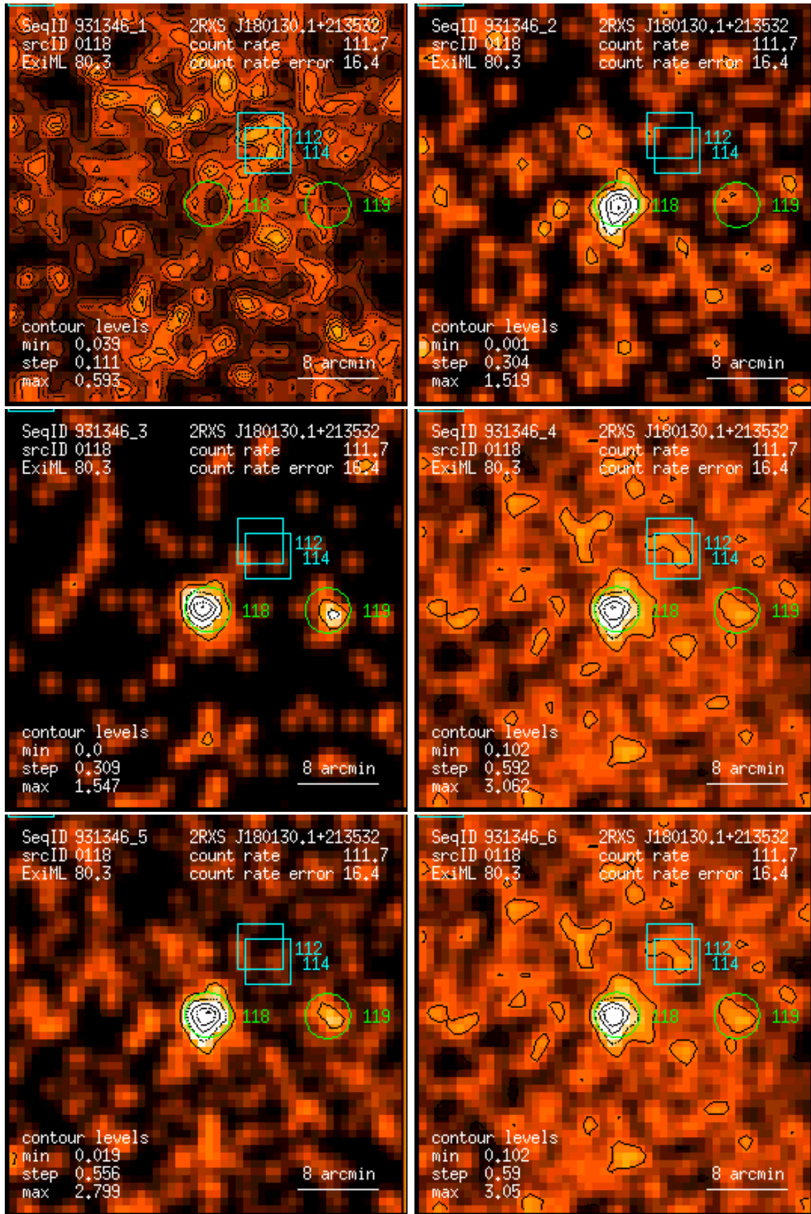
Figure 118: RASS 931346: detection 0118: band rate images, Gaussian filter: (1) PSPC channels 11 – 41, (2) 52 – 90, (3) 91 – 201, (4) 11 – 235, (5) 52 – 201, (6) 11 – 201. Broad band rates in counts/ks. Band rate contour levels in counts/ks/arcmin 2 .
