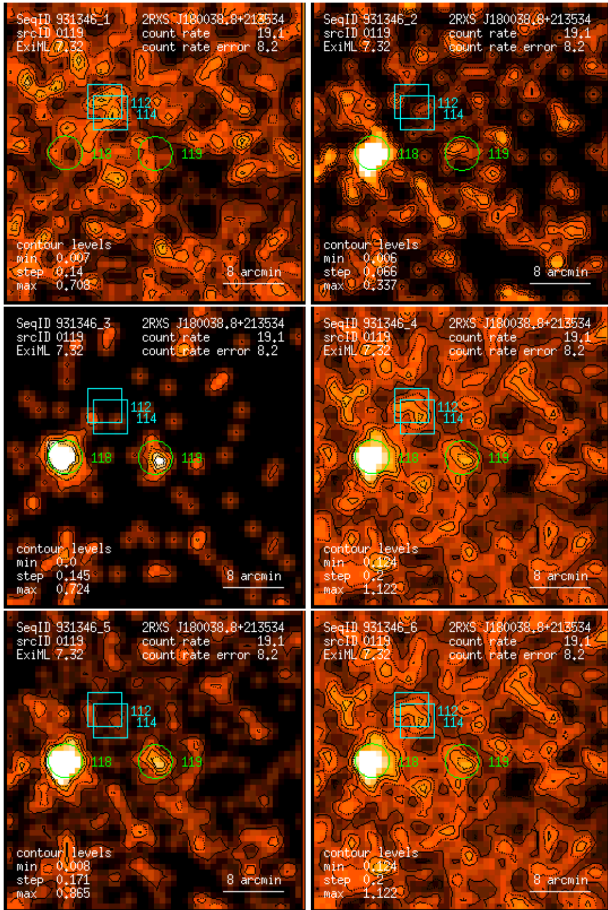
Figure 119: RASS 931346: detection 0119: band rate images, Gaussian filter: (1) PSPP channels 11 – 41, (2) 52 – 90, (3) 91 – 201, (4) 11 – 235, (5) 52 – 201, (6) 11 – 201. Broad band rates in counts/ks. Band rate contour levels in counts/ks/arcmin 2 .
