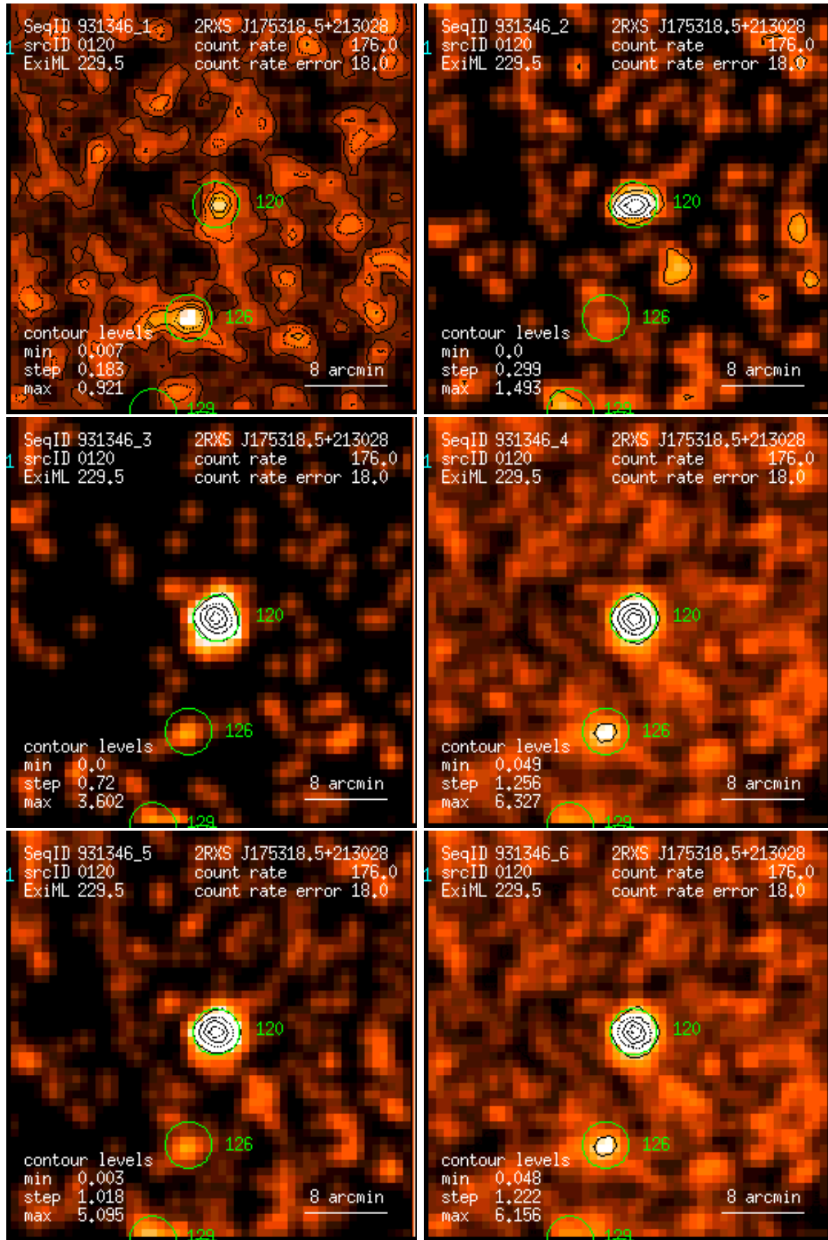
Figure 120: RASS 931346: detection 0120: band rate images, Gaussian filter: (1) PSPC channels 11 – 41, (2) 52 – 90, (3) 91 – 201, (4) 11 – 235, (5) 52 – 201, (6) 11 – 201. Broad band rates in counts/ks. Band rate contour levels in counts/ks/arcmin 2 .
