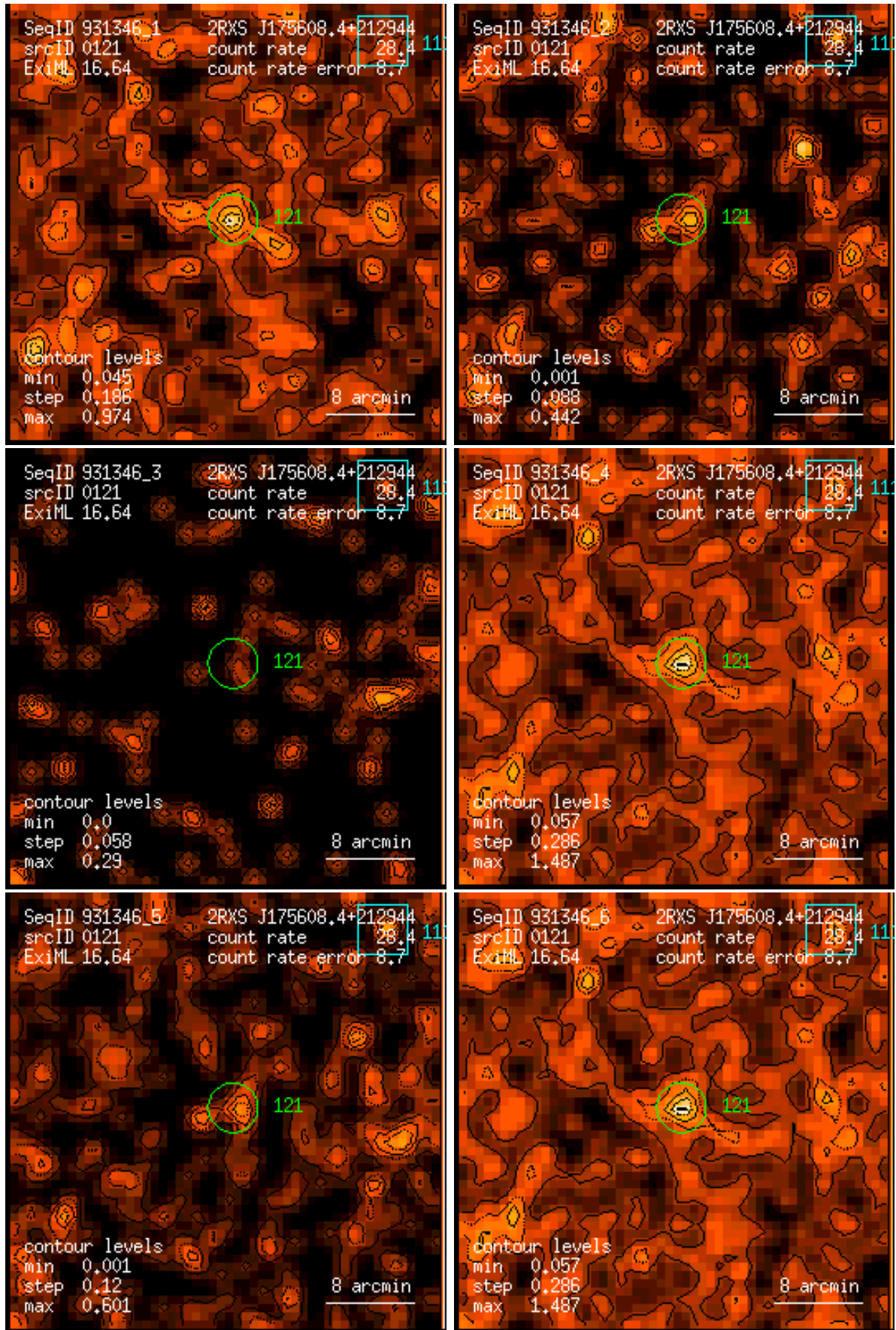
Figure 121: RASS 931346: detection 0121: band rate images, Gaussian filter: (1) PSPC channels 11 – 41, (2) 52 – 90, (3) 91 – 201, (4) 11 – 235, (5) 52 – 201, (6) 11 – 201. Broad band rates in counts/ks. Band rate contour levels in counts/ks/arcmin 2 .
