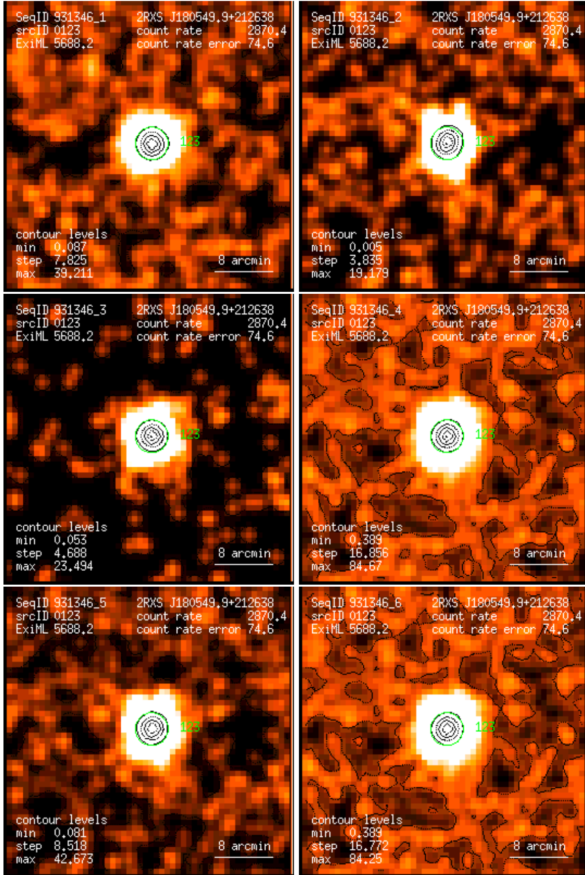
Figure 123: RASS 931346: detection 0123: band rate images, Gaussian filter: (1) PSPC channels 11 – 41, (2) 52 – 90, (3) 91 – 201, (4) 11 – 235, (5) 52 – 201, (6) 11 – 201. Broad band rates in counts/ks. Band rate contour levels in counts/ks/arcmin 2 .
