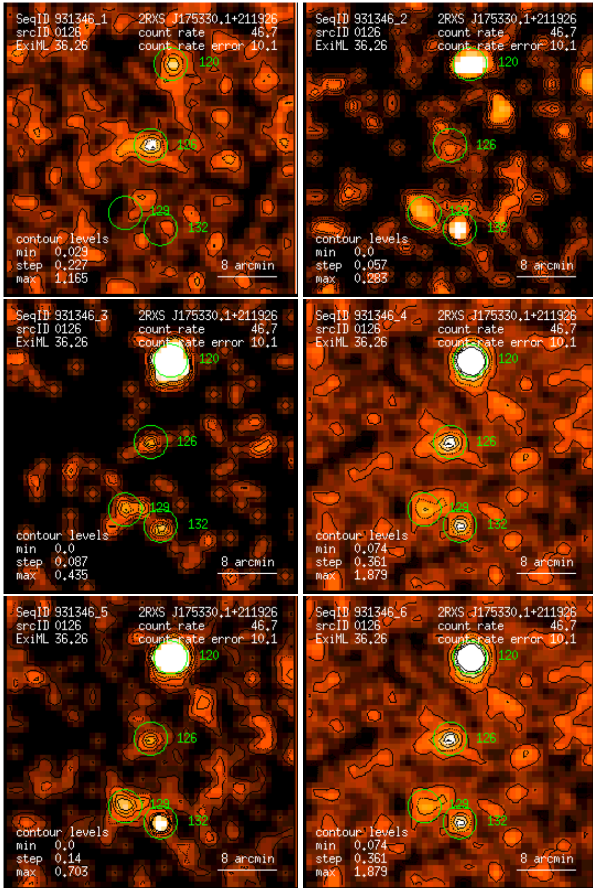
Figure 126: RASS 931346: detection 0126: band rate images, Gaussian filter: (1) PSPC channels 11 – 41, (2) 52 – 90, (3) 91 – 201, (4) 11 – 235, (5) 52 – 201, (6) 11 – 201. Broad band rates in counts/ks. Band rate contour levels in counts/ks/arcmin 2 .
