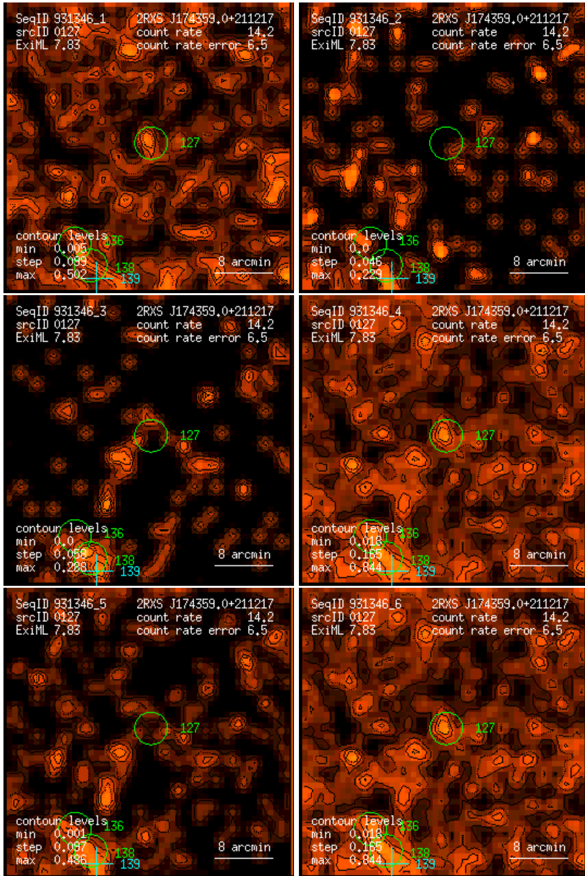
Figure 127: RASS 931346: detection 0127: band rate images, Gaussian filter: (1) PSPC channels 11 – 41, (2) 52 – 90, (3) 91 – 201, (4) 11 – 235, (5) 52 – 201, (6) 11 – 201. Broad band rates in counts/ks. Band rate contour levels in counts/ks/arcmin 2 .
