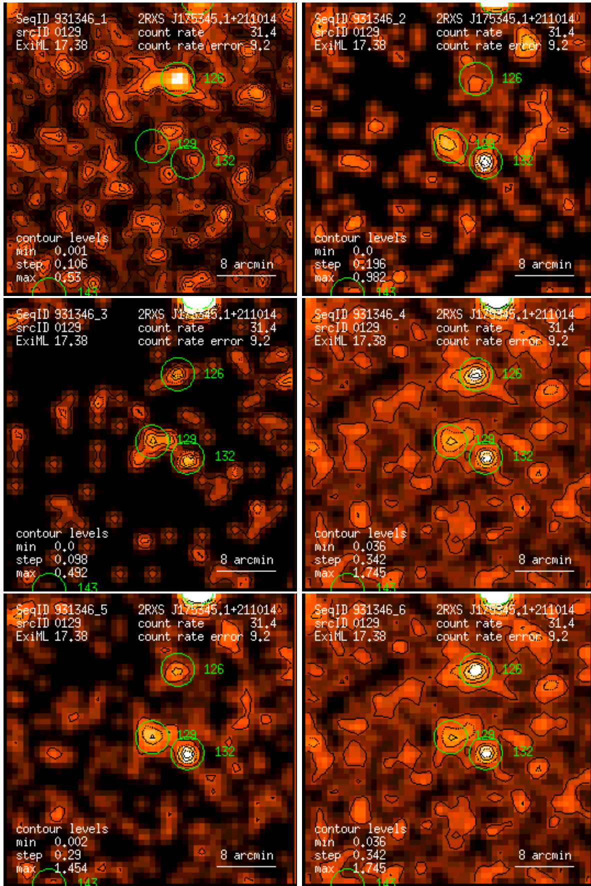
Figure 129: RASS 931346: detection 0129: band rate images, Gaussian filter: (1) PSPC channels 11 – 41, (2) 52 – 90, (3) 91 – 201, (4) 11 – 235, (5) 52 – 201, (6) 11 – 201. Broad band rates in counts/ks. Band rate contour levels in counts/ks/arcmin 2 .
