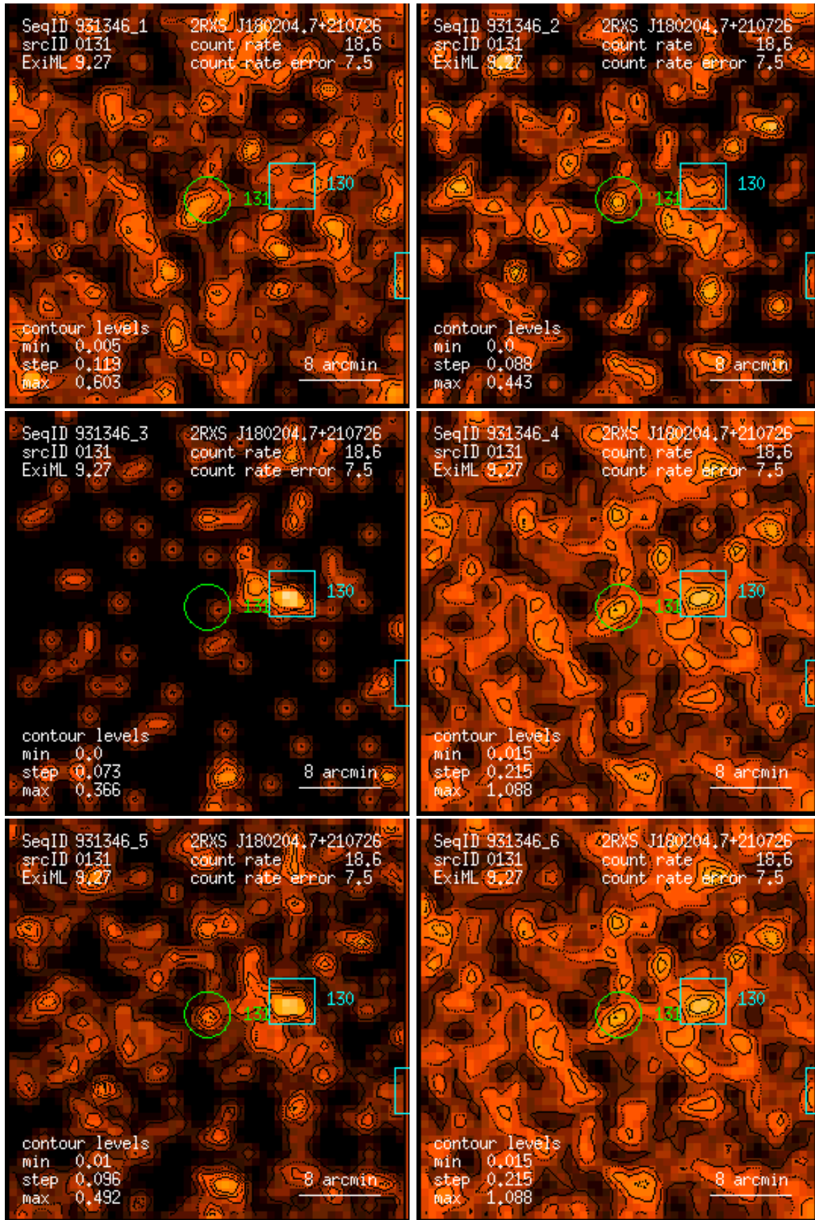
Figure 131: RASS 931346: detection 0131: band rate images, Gaussian filter: (1) PSPC channels 11 – 41, (2) 52 – 90, (3) 91 – 201, (4) 11 – 235, (5) 52 – 201, (6) 11 – 201. Broad band rates in counts/ks. Band rate contour levels in counts/ks/arcmin 2 .
