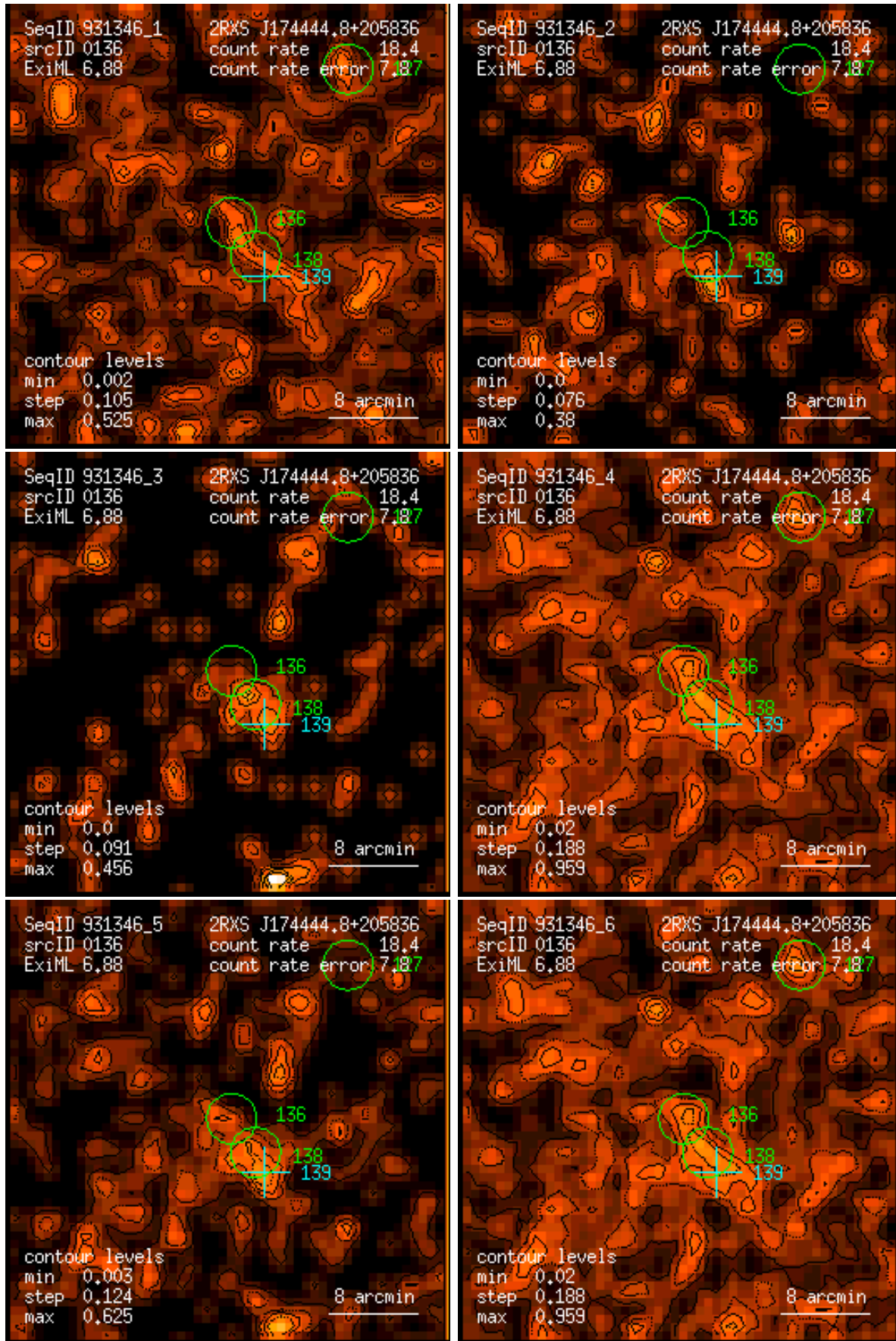
Figure 136: RASS 931346: detection 0136: band rate images, Gaussian filter: (1) PSPC channels 11 – 41, (2) 52 – 90, (3) 91 – 201, (4) 11 – 235, (5) 52 – 201, (6) 11 – 201. Broad band rates in counts/ks. Band rate contour levels in counts/ks/arcmin 2 .
