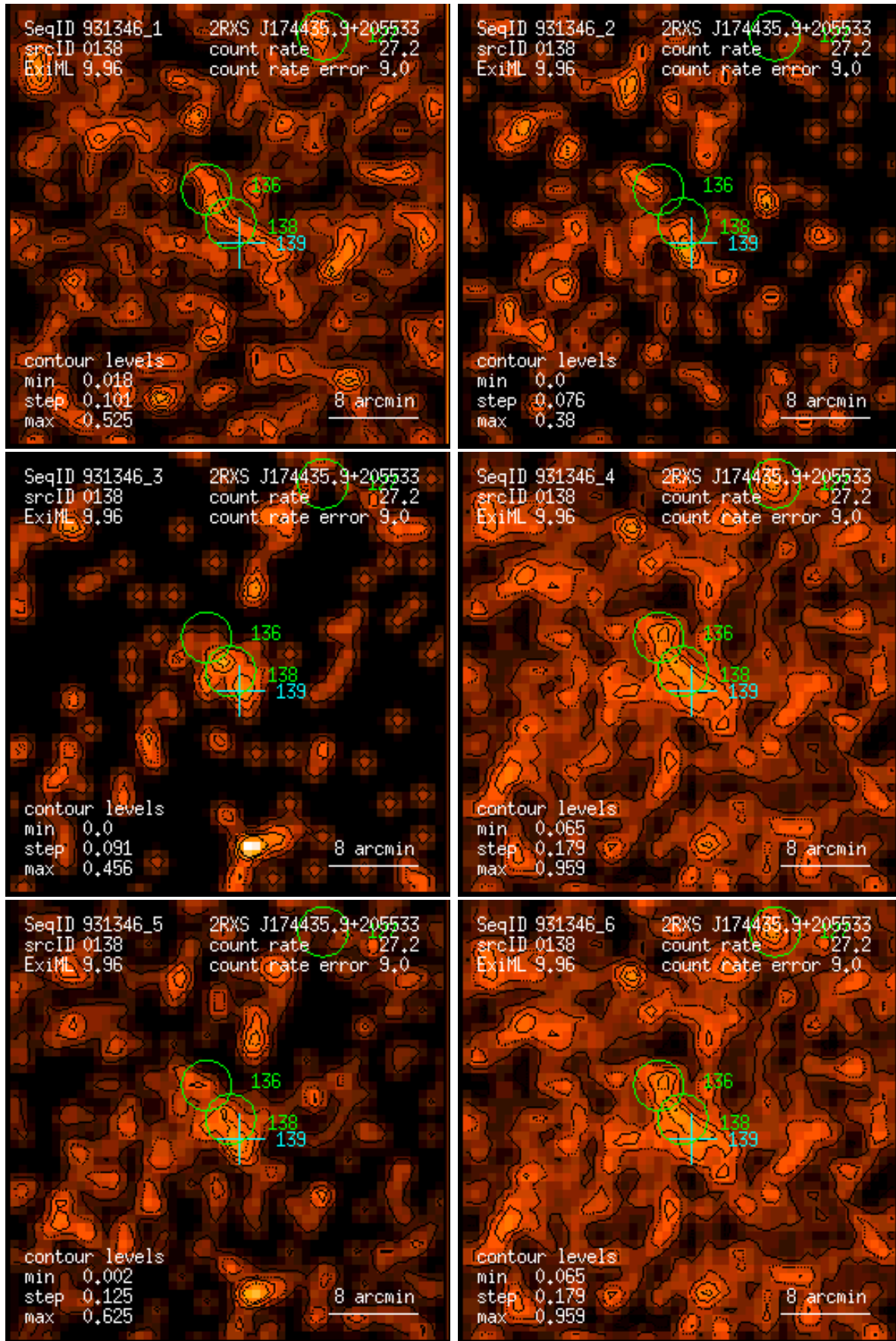
Figure 138: RASS 931346: detection 0138: band rate images, Gaussian filter: (1) PSPC channels 11 – 41, (2) 52 – 90, (3) 91 – 201, (4) 11 – 235, (5) 52 – 201, (6) 11 – 201. Broad band rates in counts/ks. Band rate contour levels in counts/ks/arcmin 2 .
