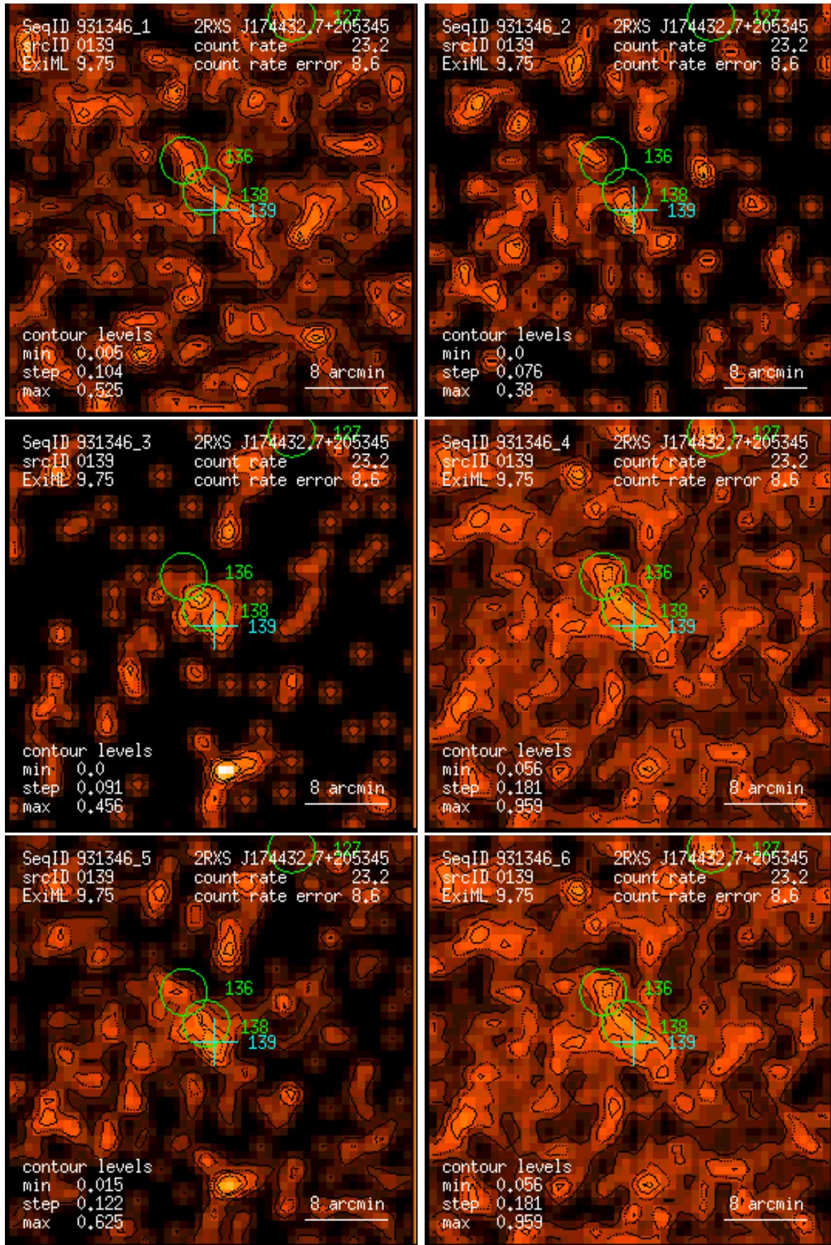
Figure 139: RASS 931346: detection 0139: band rate images, Gaussian filter: (1) PSPC channels 11 – 41, (2) 52 – 90, (3) 91 – 201, (4) 11 – 235, (5) 52 – 201, (6) 11 – 201. Broad band rates in counts/ks. Band rate contour levels in counts/ks/arcmin 2 .
