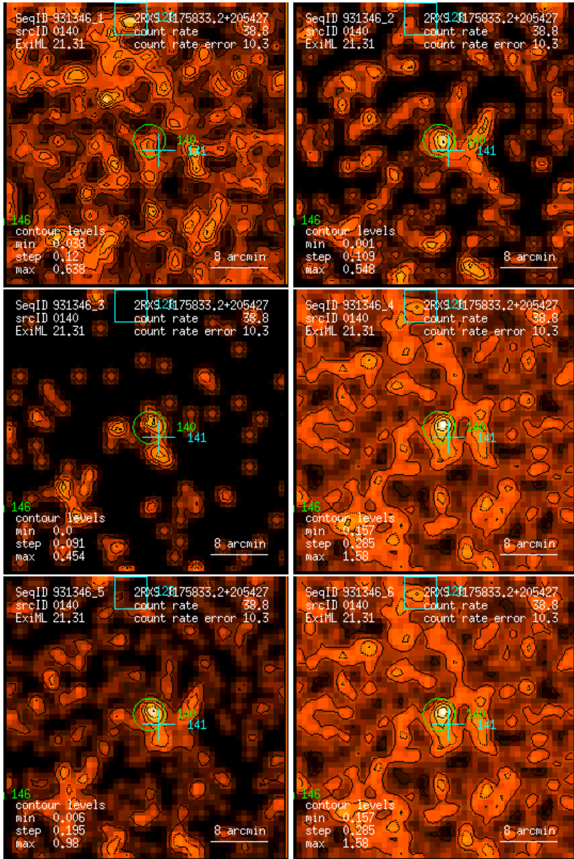
Figure 140: RASS 931346: detection 0140: band rate images, Gaussian filter: (1) PSPC channels 11 – 41, (2) 52 – 90, (3) 91 – 201, (4) 11 – 235, (5) 52 – 201, (6) 11 – 201. Broad band rates in counts/ks. Band rate contour levels in counts/ks/arcmin 2 .
