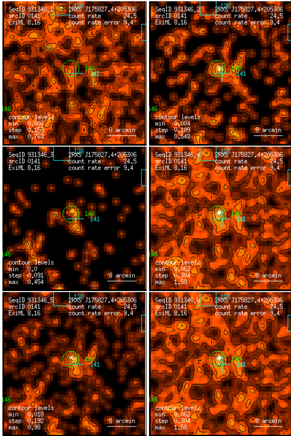
Figure 141: RASS 931346: detection 0141: band rate images, Gaussian filter: (1) PSPC channels 11 – 41, (2) 52 – 90, (3) 91 – 201, (4) 11 – 235, (5) 52 – 201, (6) 11 – 201. Broad band rates in counts/ks. Band rate contour levels in counts/ks/arcmin 2 .
