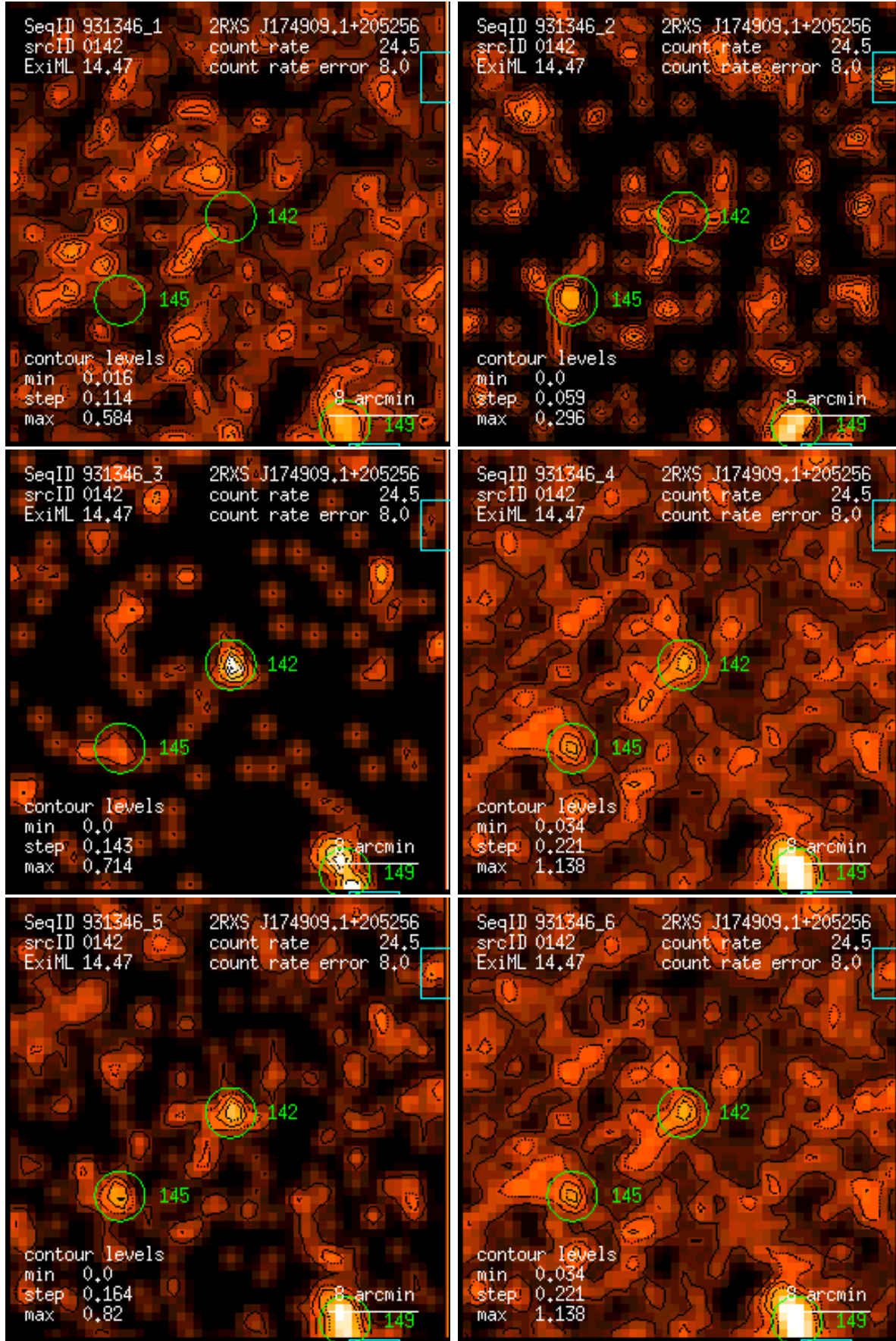
Figure 142: RASS 931346: detection 0142: band rate images, Gaussian filter: (1) PSPC channels 11 – 41, (2) 52 – 90, (3) 91 – 201, (4) 11 – 235, (5) 52 – 201, (6) 11 – 201. Broad band rates in counts/ks. Band rate contour levels in counts/ks/arcmin 2 .
