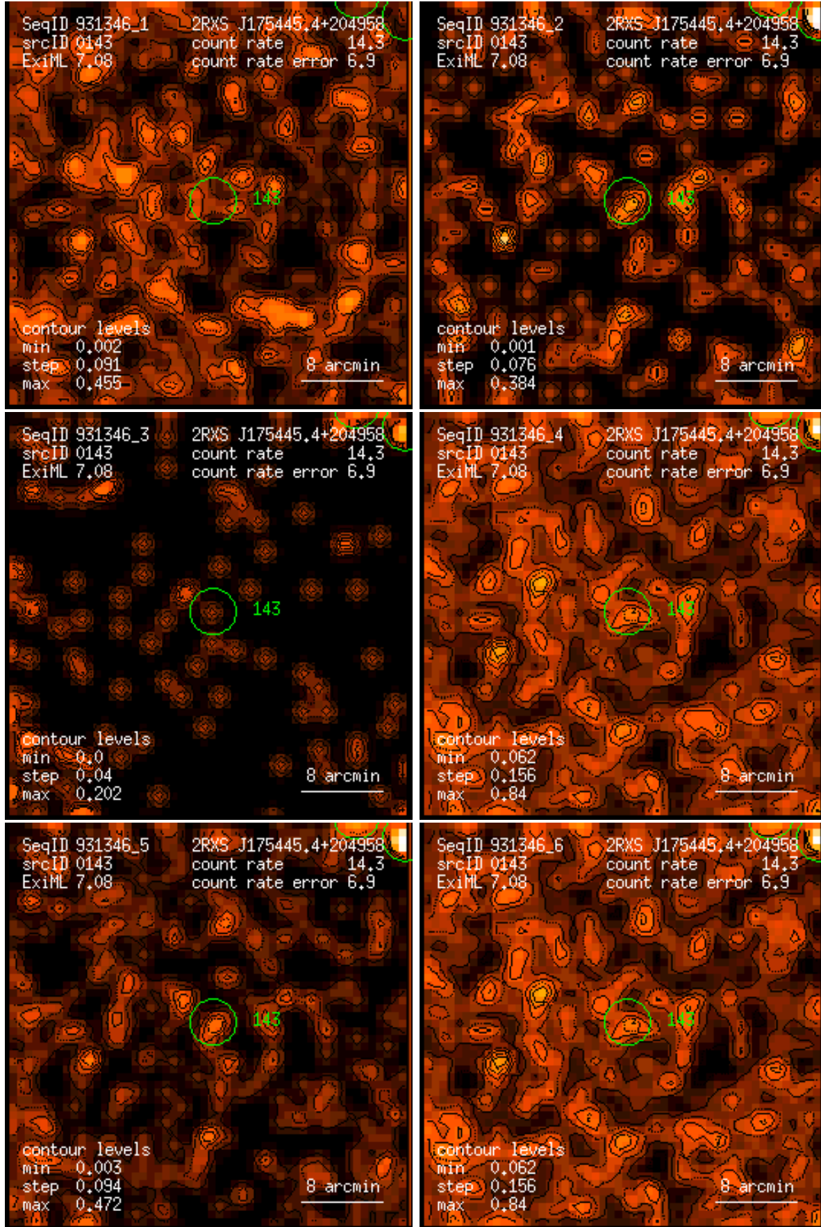
Figure 143: RASS 931346: detection 0143: band rate images, Gaussian filter: (1) PSPC channels 11 – 41, (2) 52 – 90, (3) 91 – 201, (4) 11 – 235, (5) 52 – 201, (6) 11 – 201. Broad band rates in counts/ks. Band rate contour levels in counts/ks/arcmin 2 .
