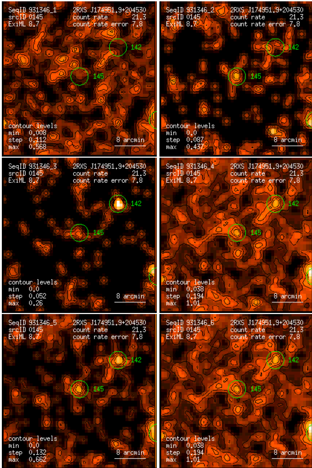
Figure 145: RASS 931346: detection 0145: band rate images, Gaussian filter: (1) PSPC channels 11 – 41, (2) 52 – 90, (3) 91 – 201, (4) 11 – 235, (5) 52 – 201, (6) 11 – 201. Broad band rates in counts/ks. Band rate contour levels in counts/ks/arcmin 2 .
