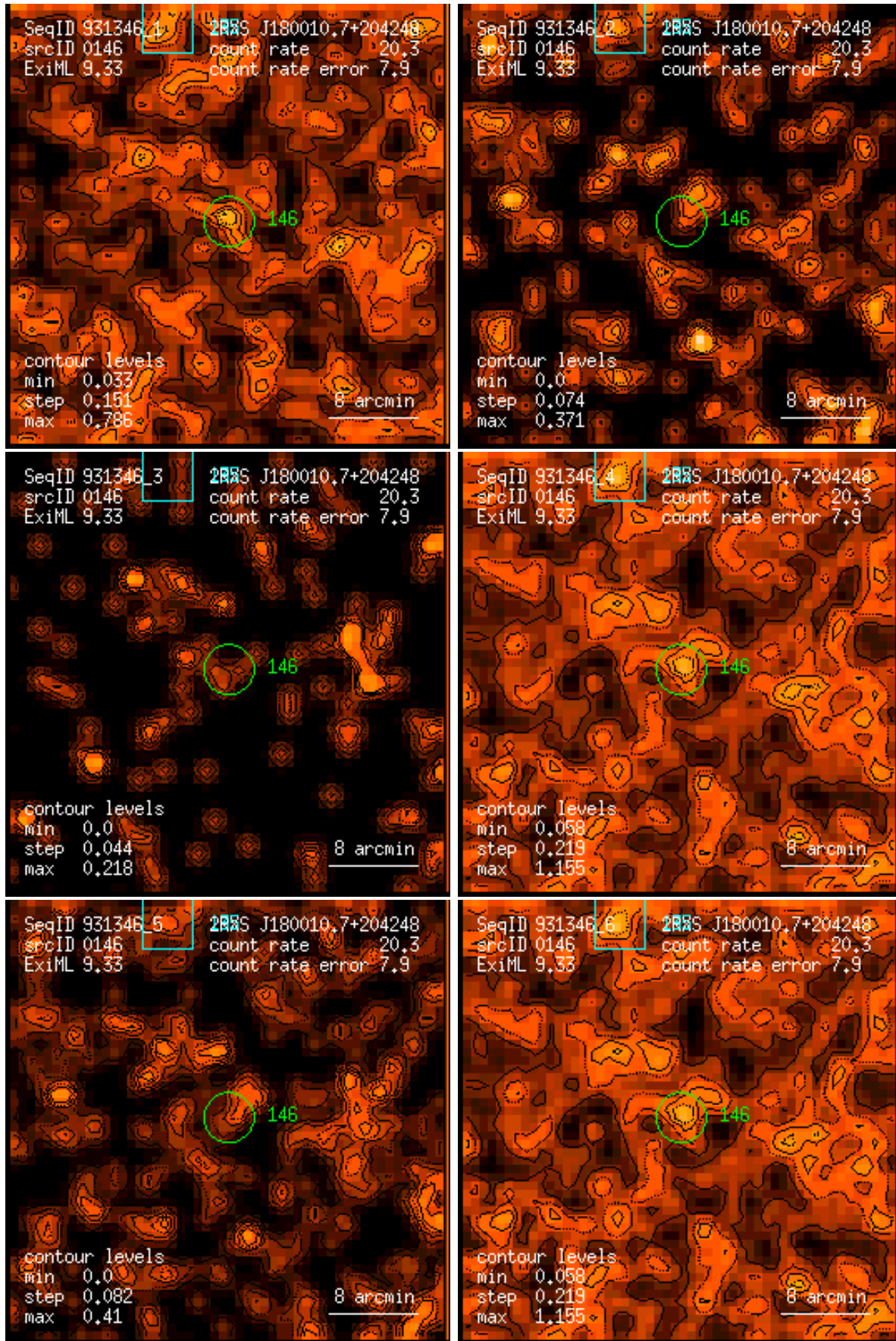
Figure 146: RASS 931346: detection 0146: band rate images, Gaussian filter: (1) PSPC channels 11 – 41, (2) 52 – 90, (3) 91 – 201, (4) 11 – 235, (5) 52 – 201, (6) 11 – 201. Broad band rates in counts/ks. Band rate contour levels in counts/ks/arcmin 2 .
