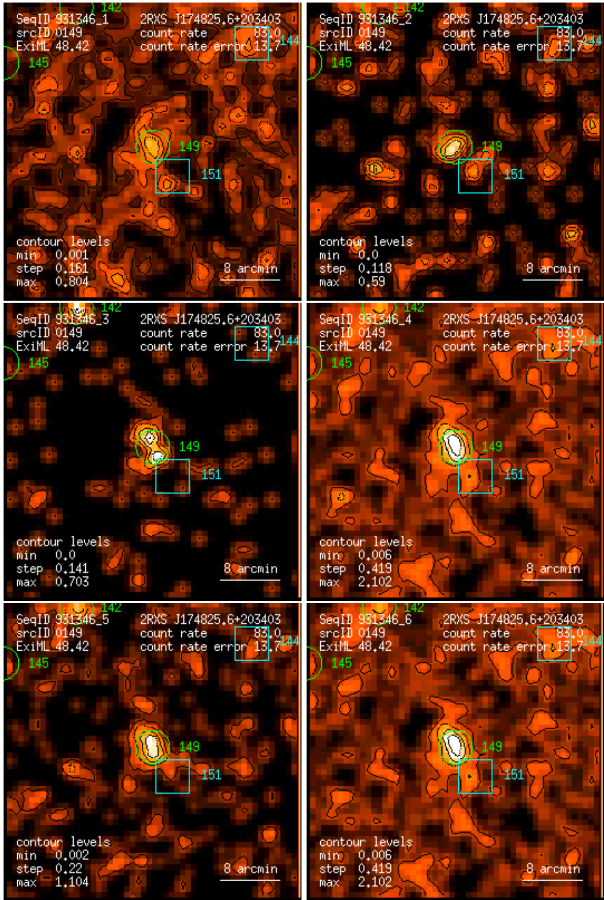
Figure 149: RASS 931346: detection 0149: band rate images, Gaussian filter: (1) PSPC channels 11 – 41, (2) 52 – 90, (3) 91 – 201, (4) 11 – 235, (5) 52 – 201, (6) 11 – 201. Broad band rates in counts/ks. Band rate contour levels in counts/ks/arcmin 2 .
