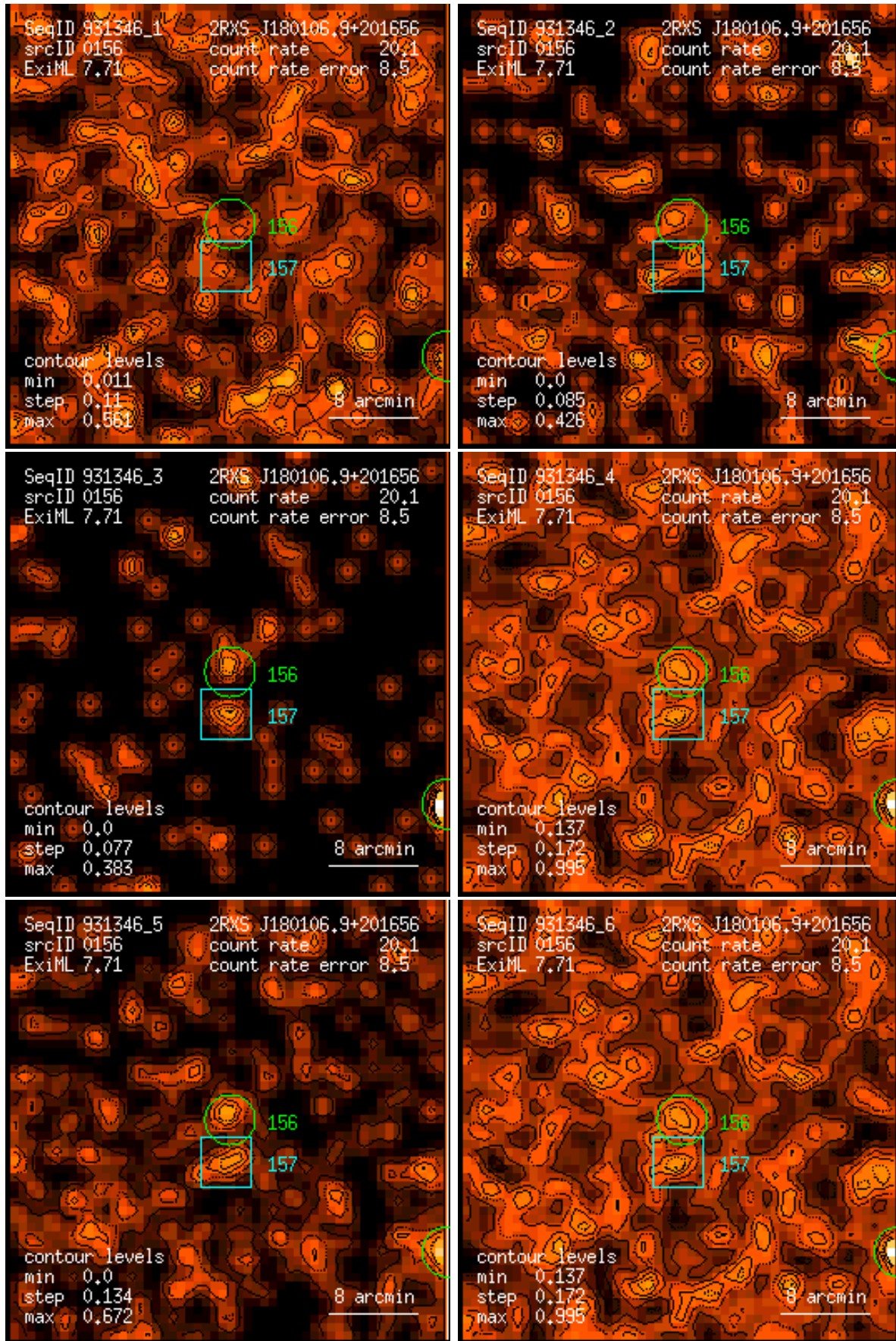
Figure 156: RASS 931346: detection 0156: band rate images, Gaussian filter: (1) PSPC channels 11 – 41, (2) 52 – 90, (3) 91 – 201, (4) 11 – 235, (5) 52 – 201, (6) 11 – 201. Broad band rates in counts/ks. Band rate contour levels in counts/ks/arcmin 2 .
