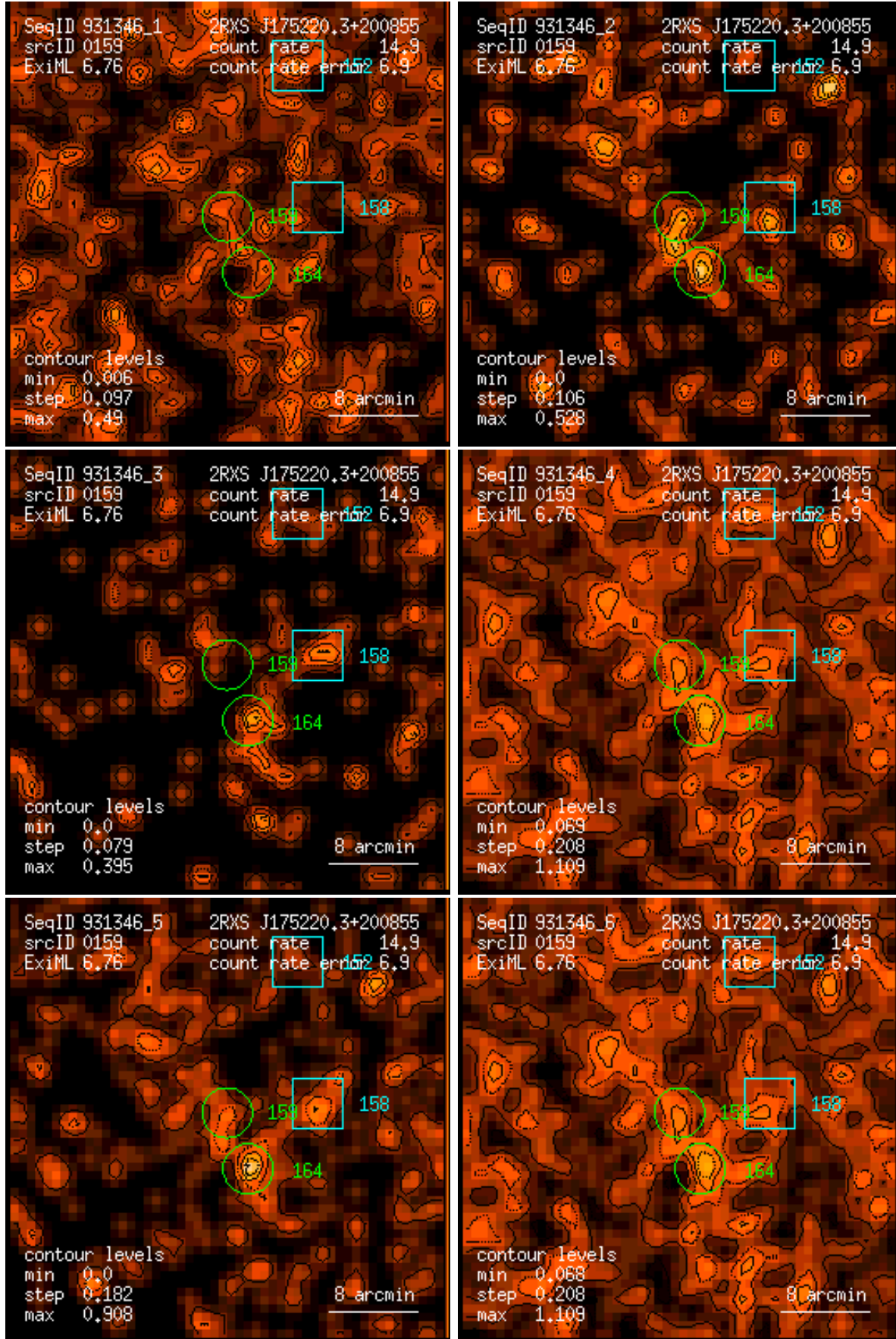
Figure 159: RASS 931346: detection 0159: band rate images, Gaussian filter: (1) PSPC channels 11 – 41, (2) 52 – 90, (3) 91 – 201, (4) 11 – 235, (5) 52 – 201, (6) 11 – 201. Broad band rates in counts/ks. Band rate contour levels in counts/ks/arcmin 2 .
