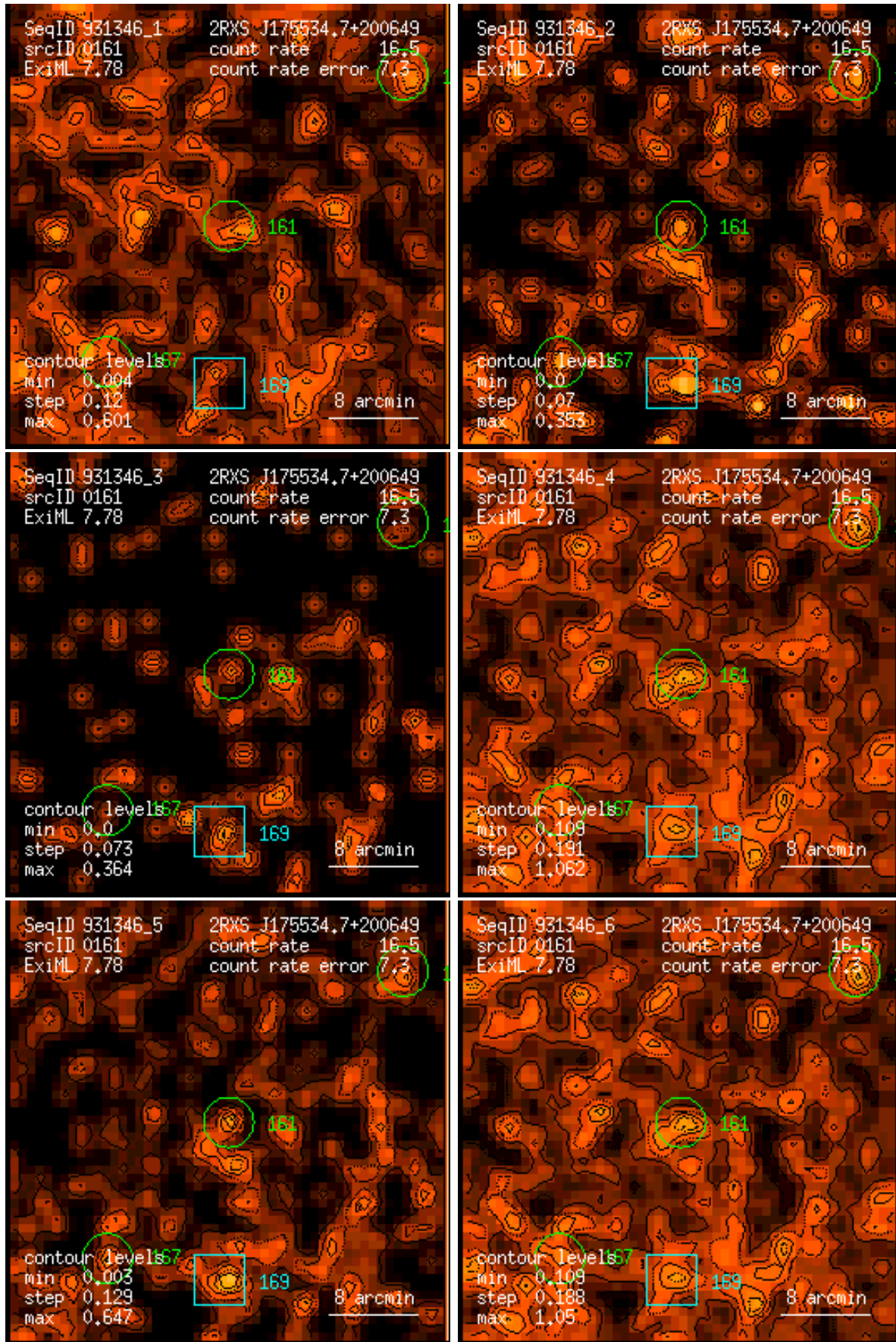
Figure 161: RASS 931346: detection 0161: band rate images, Gaussian filter: (1) PSPC channels 11 – 41, (2) 52 – 90, (3) 91 – 201, (4) 11 – 235, (5) 52 – 201, (6) 11 – 201. Broad band rates in counts/ks. Band rate contour levels in counts/ks/arcmin 2 .
