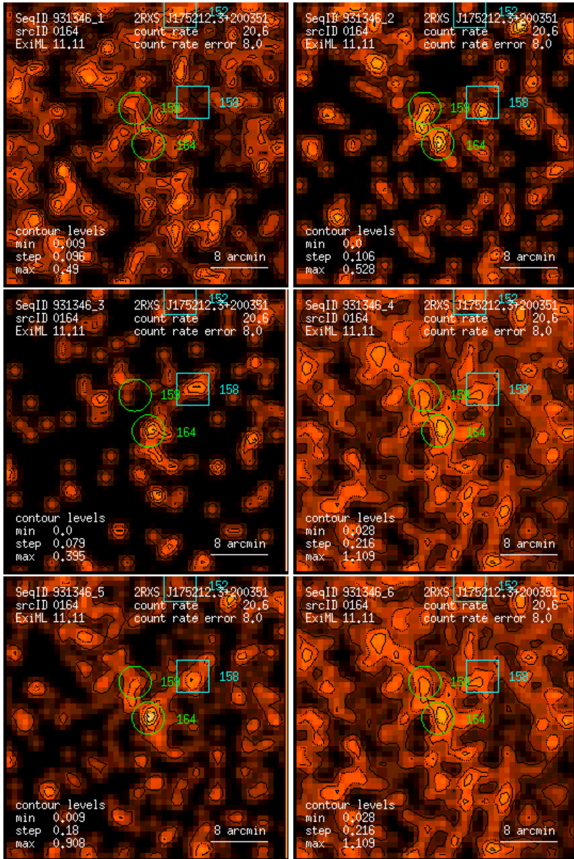
Figure 164: RASS 931346: detection 0164: band rate images, Gaussian filter: (1) PSPC channels 11 – 41, (2) 52 – 90, (3) 91 – 201, (4) 11 – 235, (5) 52 – 201, (6) 11 – 201. Broad band rates in counts/ks. Band rate contour levels in counts/ks/arcmin 2 .
