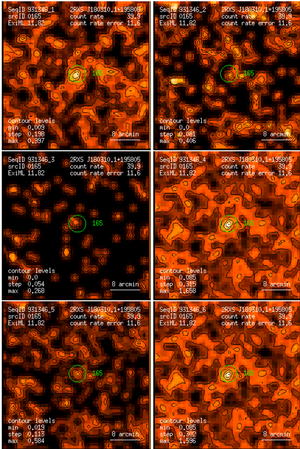
Figure 165: RASS 931346: detection 0165: band rate images, Gaussian filter: (1) PSPC channels 11 – 41, (2) 52 – 90, (3) 91 – 201, (4) 11 – 235, (5) 52 – 201, (6) 11 – 201. Broad band rates in counts/ks. Band rate contour levels in counts/ks/arcmin 2 .
