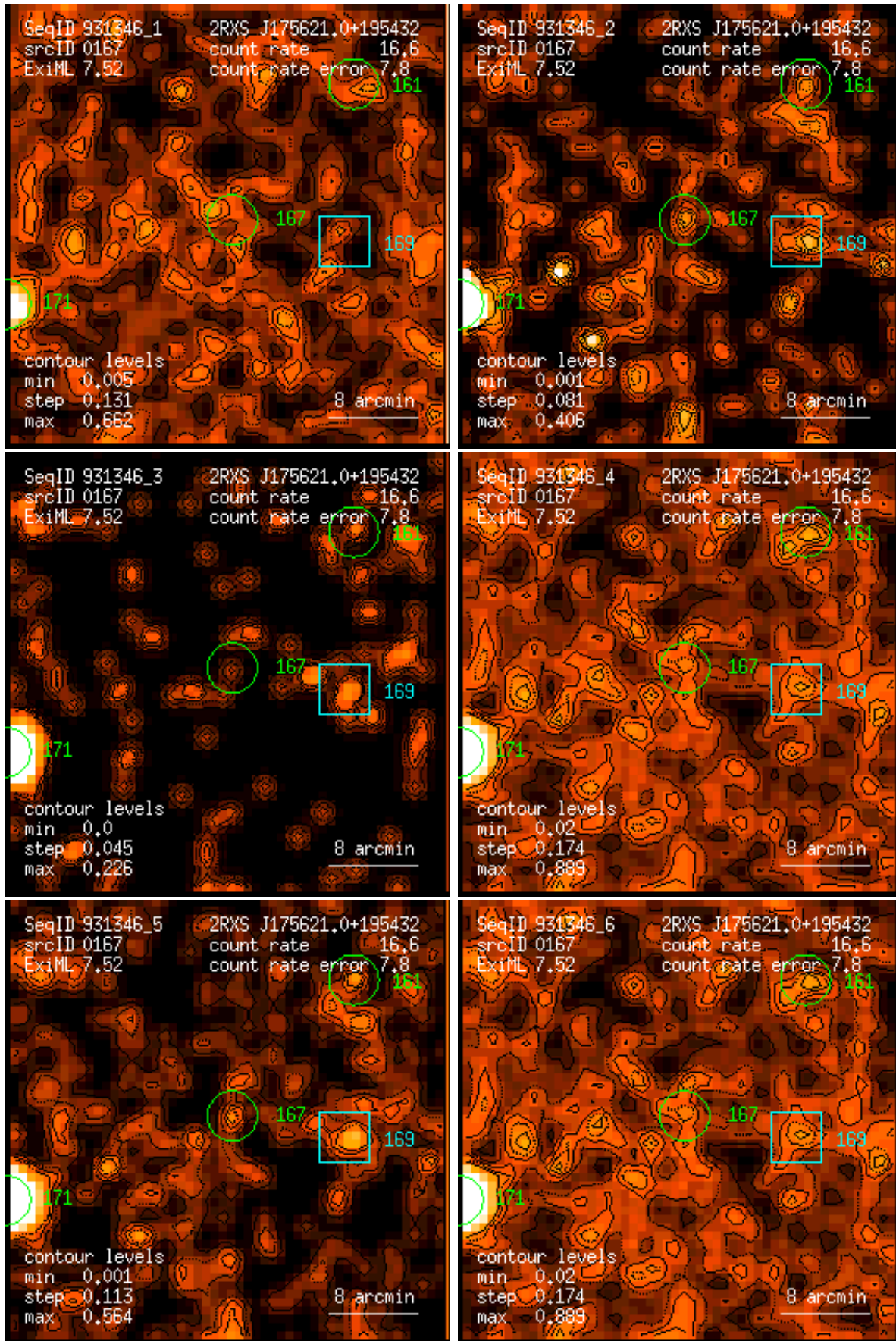
Figure 167: RASS 931346: detection 0167: band rate images, Gaussian filter: (1) PSPC channels 11 – 41, (2) 52 – 90, (3) 91 – 201, (4) 11 – 235, (5) 52 – 201, (6) 11 – 201. Broad band rates in counts/ks. Band rate contour levels in counts/ks/arcmin 2 .
