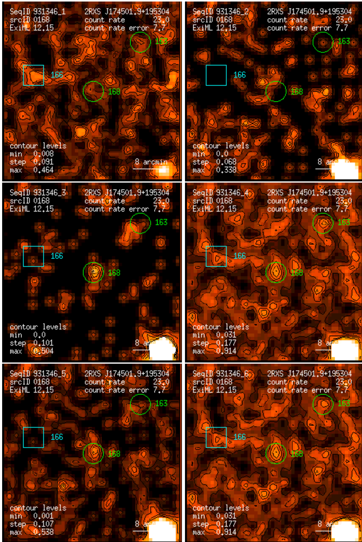
Figure 168: RASS 931346: detection 0168: band rate images, Gaussian filter: (1) PSPC channels 11 – 41, (2) 52 – 90, (3) 91 – 201, (4) 11 – 235, (5) 52 – 201, (6) 11 – 201. Broad band rates in counts/ks. Band rate contour levels in counts/ks/arcmin 2 .
