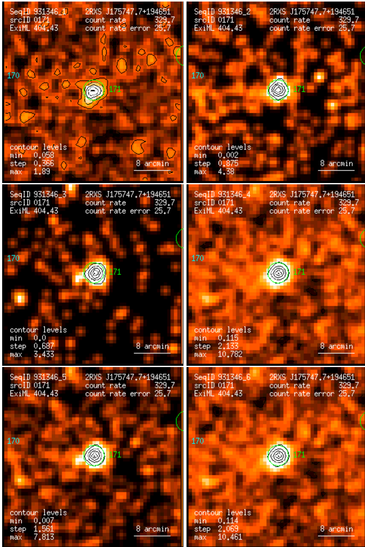
Figure 171: RASS 931346: detection 0171: band rate images, Gaussian filter: (1) PSPC channels 11 – 41, (2) 52 – 90, (3) 91 – 201, (4) 11 – 235, (5) 52 – 201, (6) 11 – 201. Broad band rates in counts/ks. Band rate contour levels in counts/ks/arcmin 2 .
