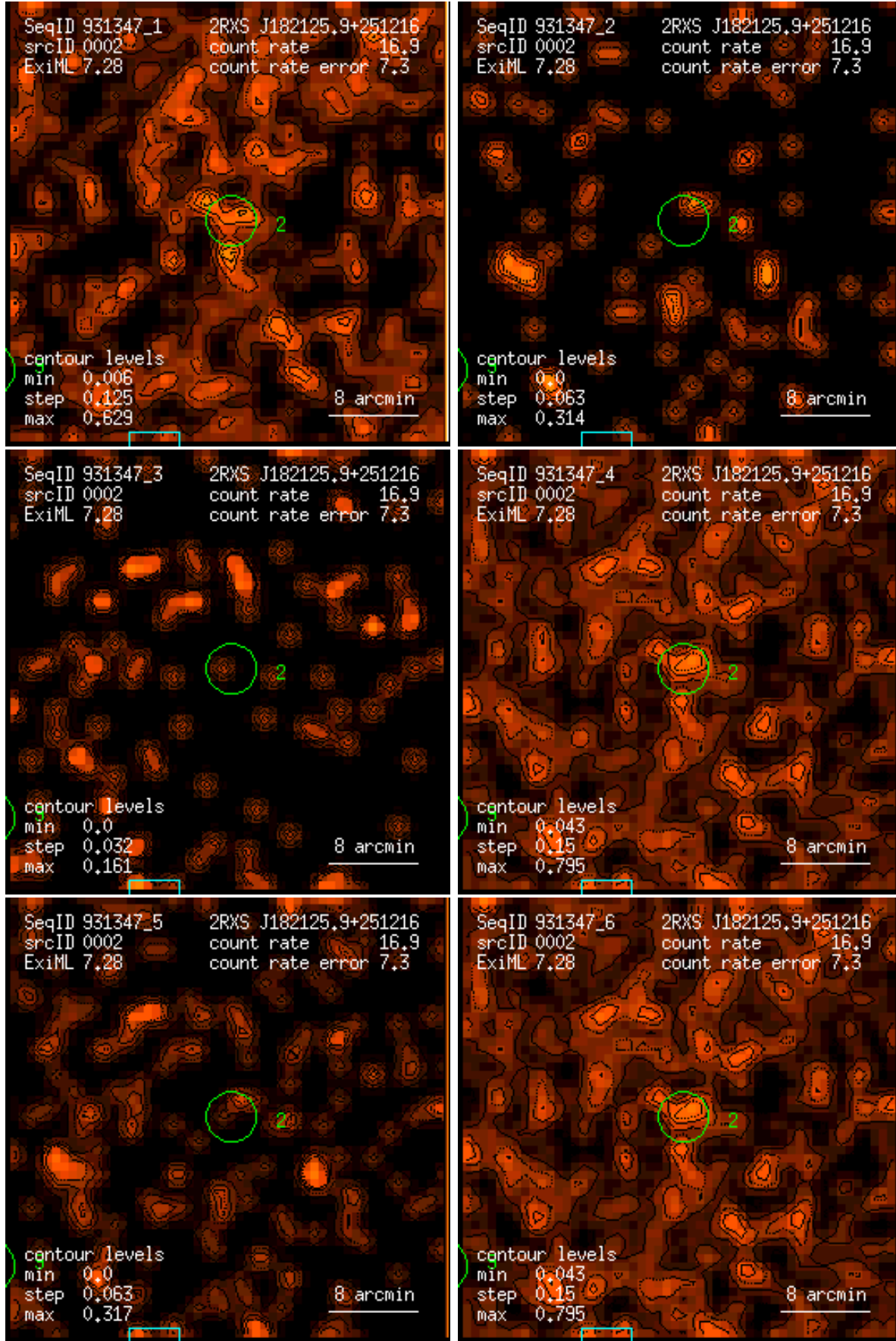
Figure 2: RASS 931347: detection 0002: band rate images, Gaussian filter: (1) PSPC channels 11 – 41, (2) 52 – 90, (3) 91 – 201, (4) 11 – 235, (5) 52 – 201, (6) 11 – 201. Broad band rates in counts/ks. Band rate contour levels in counts/ks/arcmin 2 .
