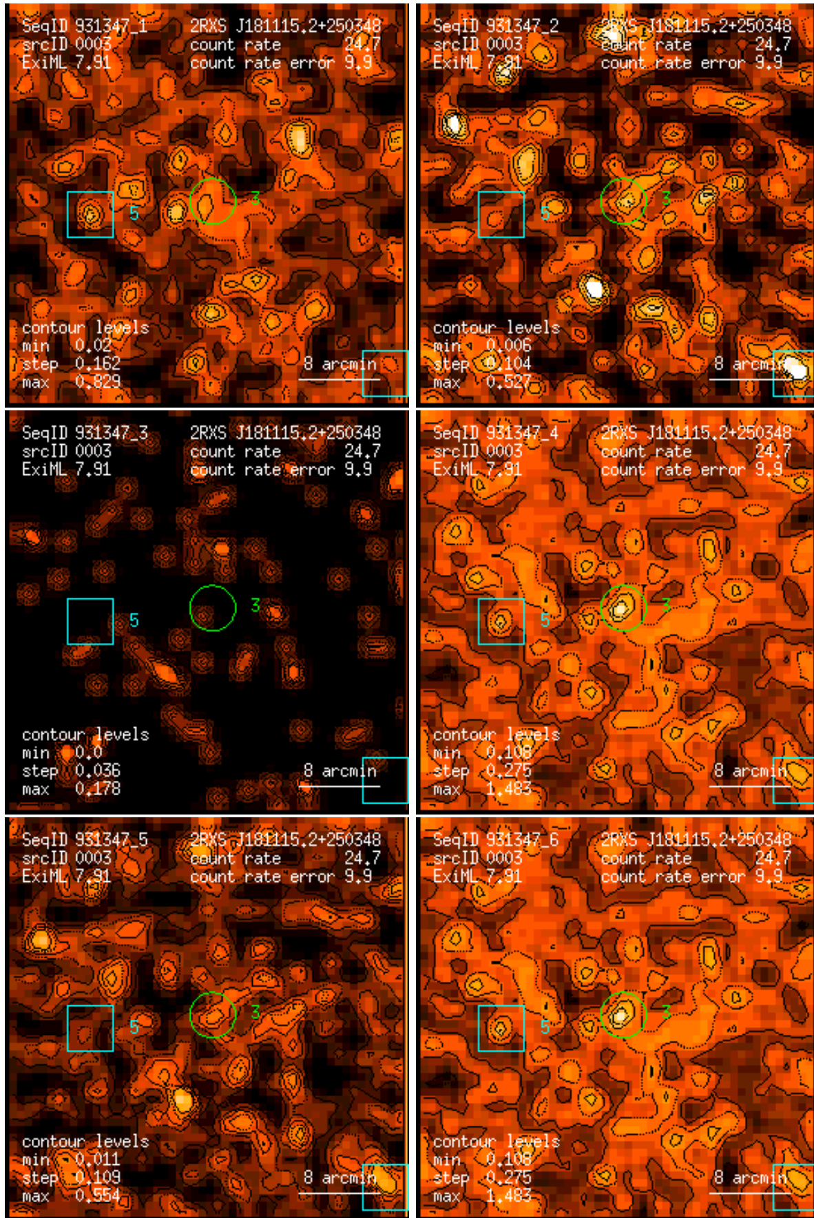
Figure 3: RASS 931347: detection 0003: band rate images, Gaussian filter: (1) PSPC channels 11 – 41, (2) 52 – 90, (3) 91 – 201, (4) 11 – 235, (5) 52 – 201, (6) 11 – 201. Broad band rates in counts/ks. Band rate contour levels in counts/ks/arcmin 2 .
