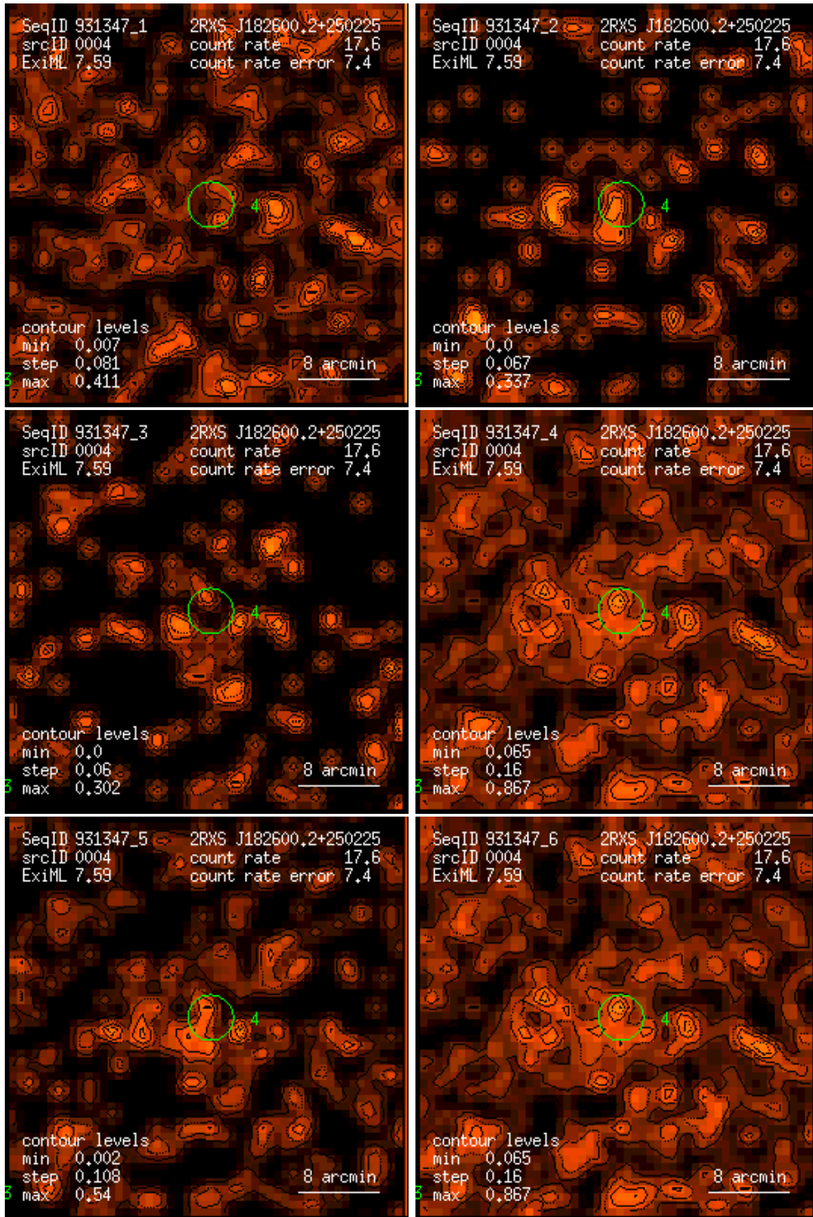
Figure 4: RASS 931347: detection 0004: band rate images, Gaussian filter: (1) PSPC channels 11 – 41, (2) 52 – 90, (3) 91 – 201, (4) 11 – 235, (5) 52 – 201, (6) 11 – 201. Broad band rates in counts/ks. Band rate contour levels in counts/ks/arcmin 2 .
