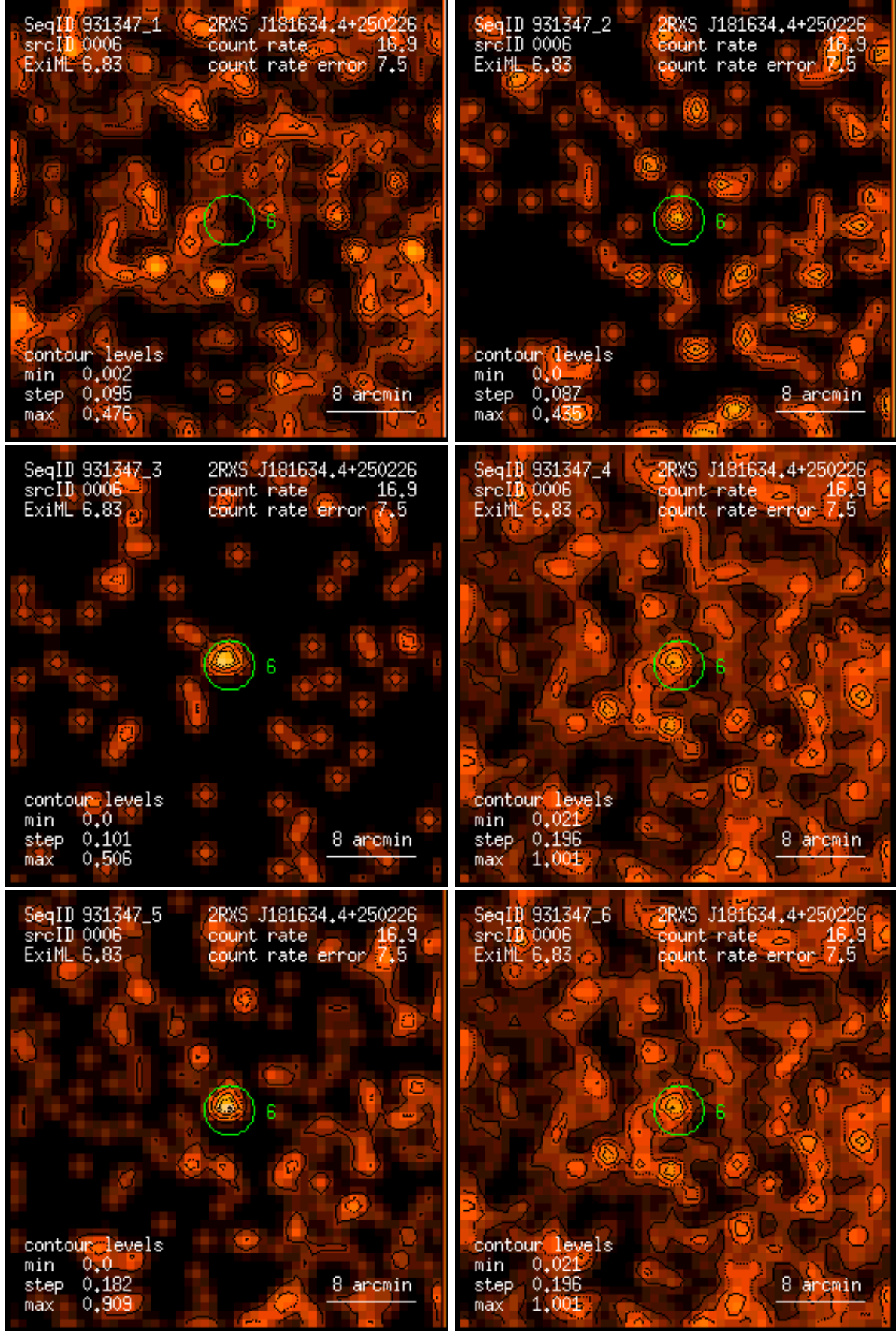
Figure 6: RASS 931347: detection 0006: band rate images, Gaussian filter: (1) PSPC channels 11 – 41, (2) 52 – 90, (3) 91 – 201, (4) 11 – 235, (5) 52 – 201, (6) 11 – 201. Broad band rates in counts/ks. Band rate contour levels in counts/ks/arcmin 2 .
