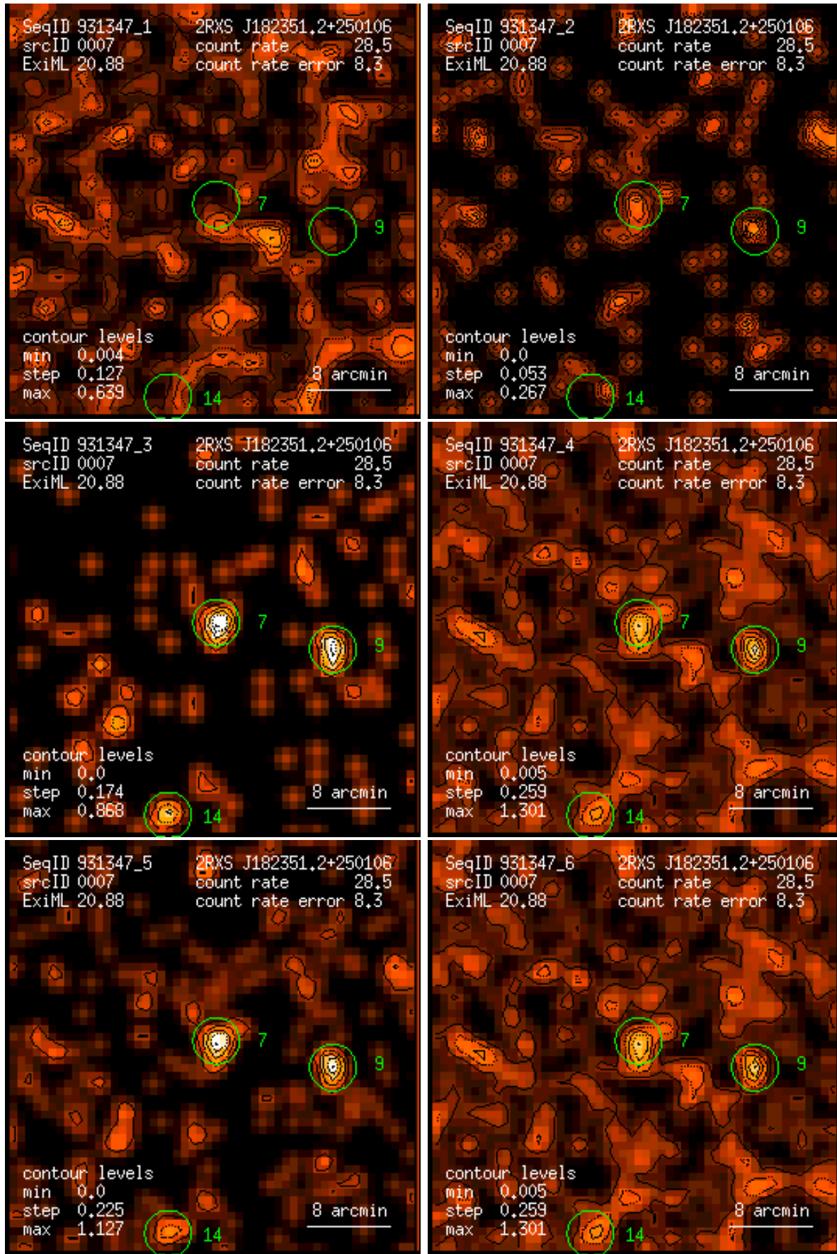
Figure 7: RASS 931347: detection 0007: band rate images, Gaussian filter: (1) PSPC channels 11 – 41, (2) 52 – 90, (3) 91 – 201, (4) 11 – 235, (5) 52 – 201, (6) 11 – 201. Broad band rates in counts/ks. Band rate contour levels in counts/ks/arcmin 2 .
