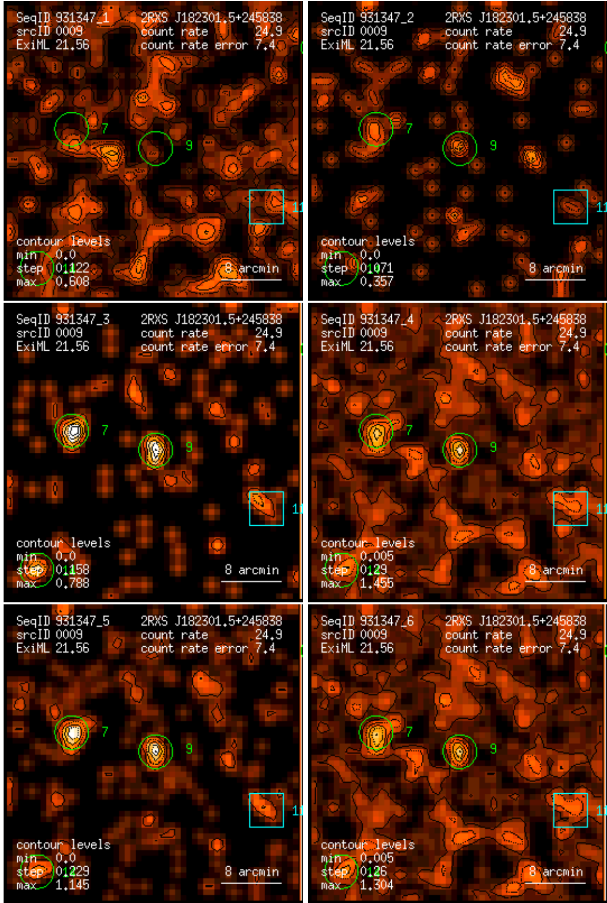
Figure 9: RASS 931347: detection 0009: band rate images, Gaussian filter: (1) PSPC channels 11 – 41, (2) 52 – 90, (3) 91 – 201, (4) 11 – 235, (5) 52 – 201, (6) 11 – 201. Broad band rates in counts/ks. Band rate contour levels in counts/ks/arcmin 2 .
