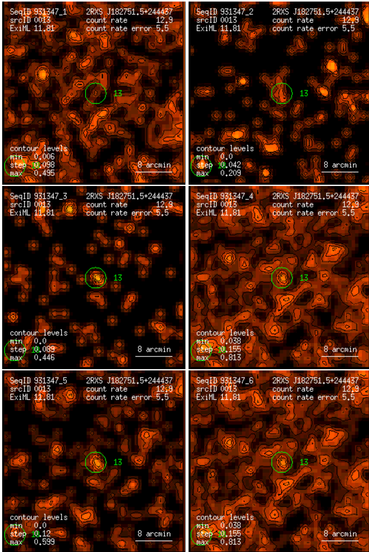
Figure 13: RASS 931347: detection 0013: band rate images, Gaussian filter: (1) PSPC channels 11 – 41, (2) 52 – 90, (3) 91 – 201, (4) 11 – 235, (5) 52 – 201, (6) 11 – 201. Broad band rates in counts/ks. Band rate contour levels in counts/ks/arcmin 2 .
