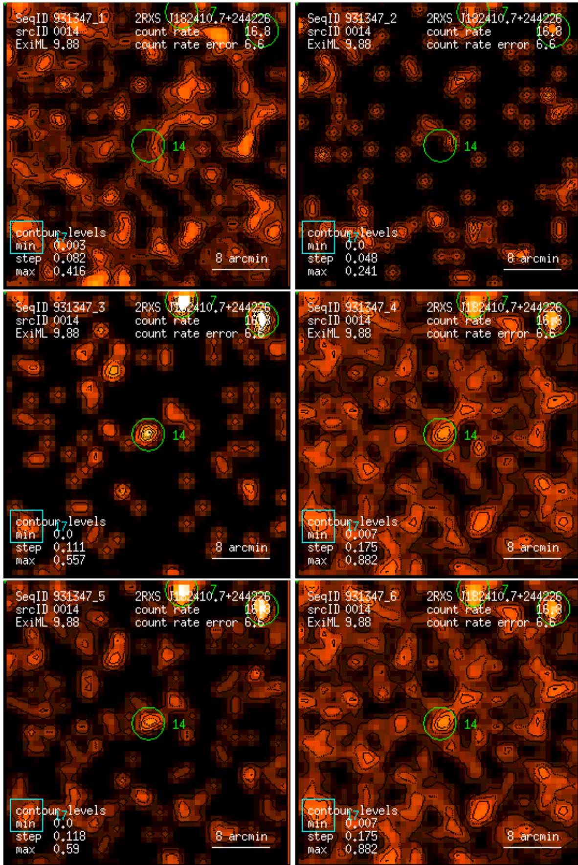
Figure 14: RASS 931347: detection 0014: band rate images, Gaussian filter: (1) PSPC channels 11 – 41, (2) 52 – 90, (3) 91 – 201, (4) 11 – 235, (5) 52 – 201, (6) 11 – 201. Broad band rates in counts/ks. Band rate contour levels in counts/ks/arcmin 2 .
