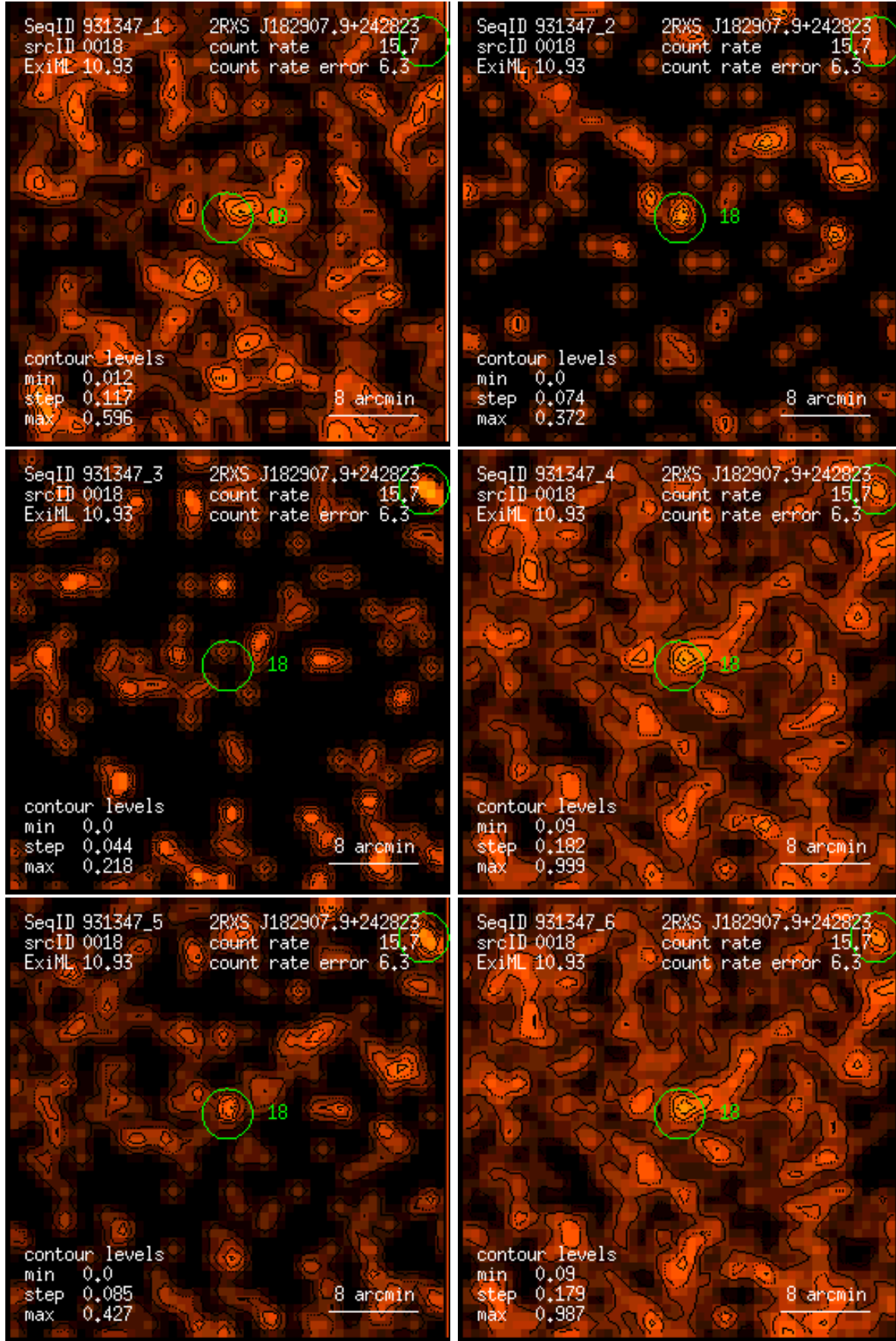
Figure 18: RASS 931347: detection 0018: band rate images, Gaussian filter: (1) PSPC channels 11 – 41, (2) 52 – 90, (3) 91 – 201, (4) 11 – 235, (5) 52 – 201, (6) 11 – 201. Broad band rates in counts/ks. Band rate contour levels in counts/ks/arcmin 2 .
