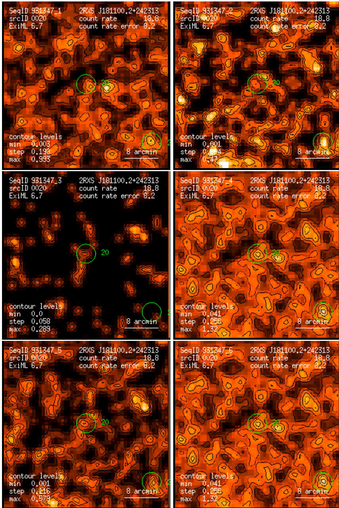
Figure 20: RASS 931347: detection 0020: band rate images, Gaussian filter: (1) PSPC channels 11 – 41, (2) 52 – 90, (3) 91 – 201, (4) 11 – 235, (5) 52 – 201, (6) 11 – 201. Broad band rates in counts/ks. Band rate contour levels in counts/ks/arcmin 2 .
