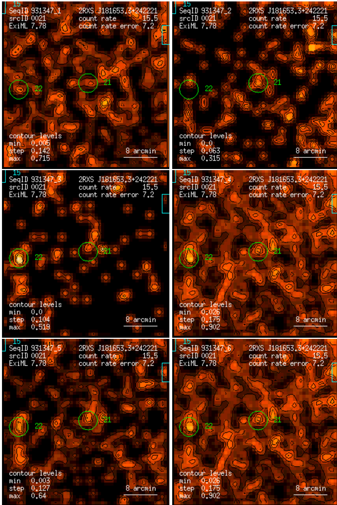
Figure 21: RASS 931347: detection 0021: band rate images, Gaussian filter: (1) PSPC channels 11 – 41, (2) 52 – 90, (3) 91 – 201, (4) 11 – 235, (5) 52 – 201, (6) 11 – 201. Broad band rates in counts/ks. Band rate contour levels in counts/ks/arcmin 2 .
