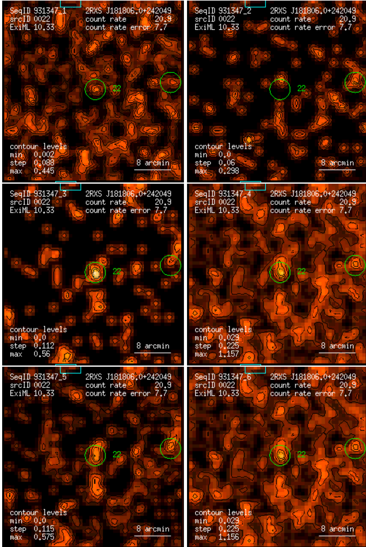
Figure 22: RASS 931347: detection 0022: band rate images, Gaussian filter: (1) PSPC channels 11 – 41, (2) 52 – 90, (3) 91 – 201, (4) 11 – 235, (5) 52 – 201, (6) 11 – 201. Broad band rates in counts/ks. Band rate contour levels in counts/ks/arcmin 2 .
